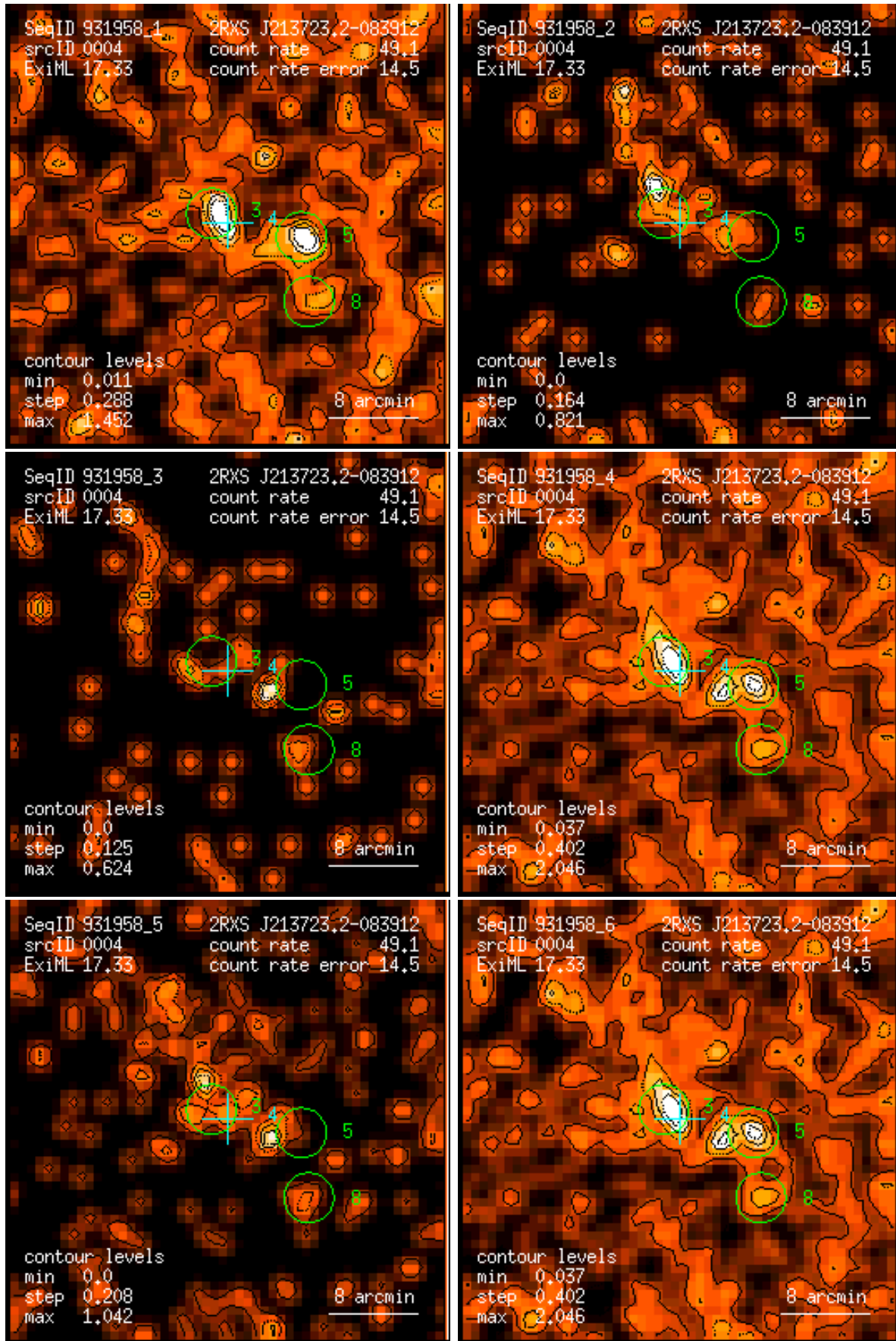
Figure 4: RASS 931958: detection 0004: band rate images, Gaussian filter: (1) PSPC channels 11 – 41, (2) 52 – 90, (3) 91 – 201, (4) 11 – 235, (5) 52 – 201, (6) 11 – 201. Broad band rates in counts/ks. Band rate contour levels in counts/ks/arcmin 2 .
