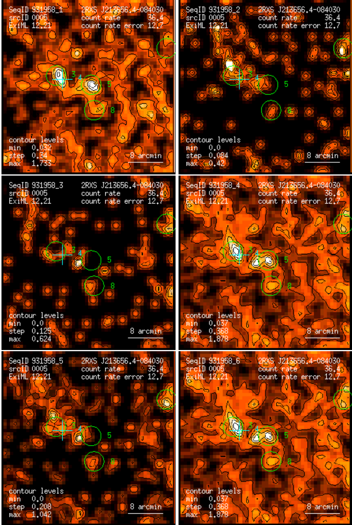
Figure 5: RASS 931958: detection 0005: band rate images, Gaussian filter: (1) PSPC channels 11 – 41, (2) 52 – 90, (3) 91 – 201, (4) 11 – 235, (5) 52 – 201, (6) 11 – 201. Broad band rates in counts/ks. Band rate contour levels in counts/ks/arcmin 2 .
