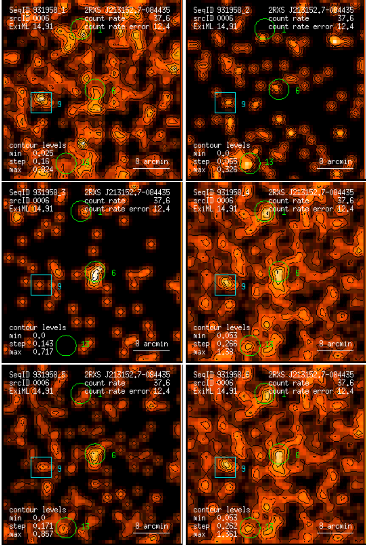
Figure 6: RASS 931958: detection 0006: band rate images, Gaussian filter: (1) PSPC channels 11 – 41, (2) 52 – 90, (3) 91 – 201, (4) 11 – 235, (5) 52 – 201, (6) 11 – 201. Broad band rates in counts/ks. Band rate contour levels in counts/ks/arcmin 2 .
