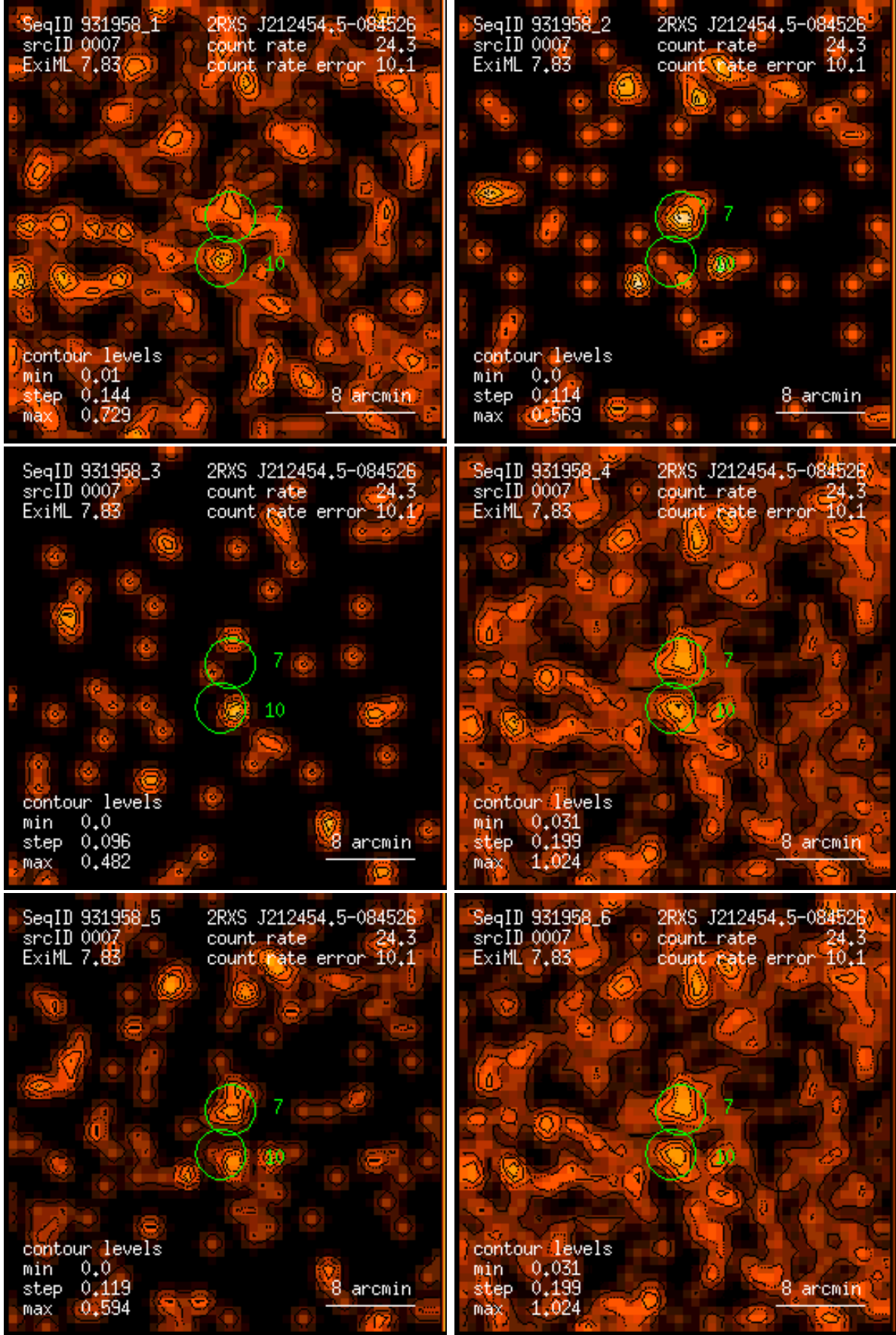
Figure 7: RASS 931958: detection 0007: band rate images, Gaussian filter: (1) PSPC channels 11 – 41, (2) 52 – 90, (3) 91 – 201, (4) 11 – 235, (5) 52 – 201, (6) 11 – 201. Broad band rates in counts/ks. Band rate contour levels in counts/ks/arcmin 2 .
