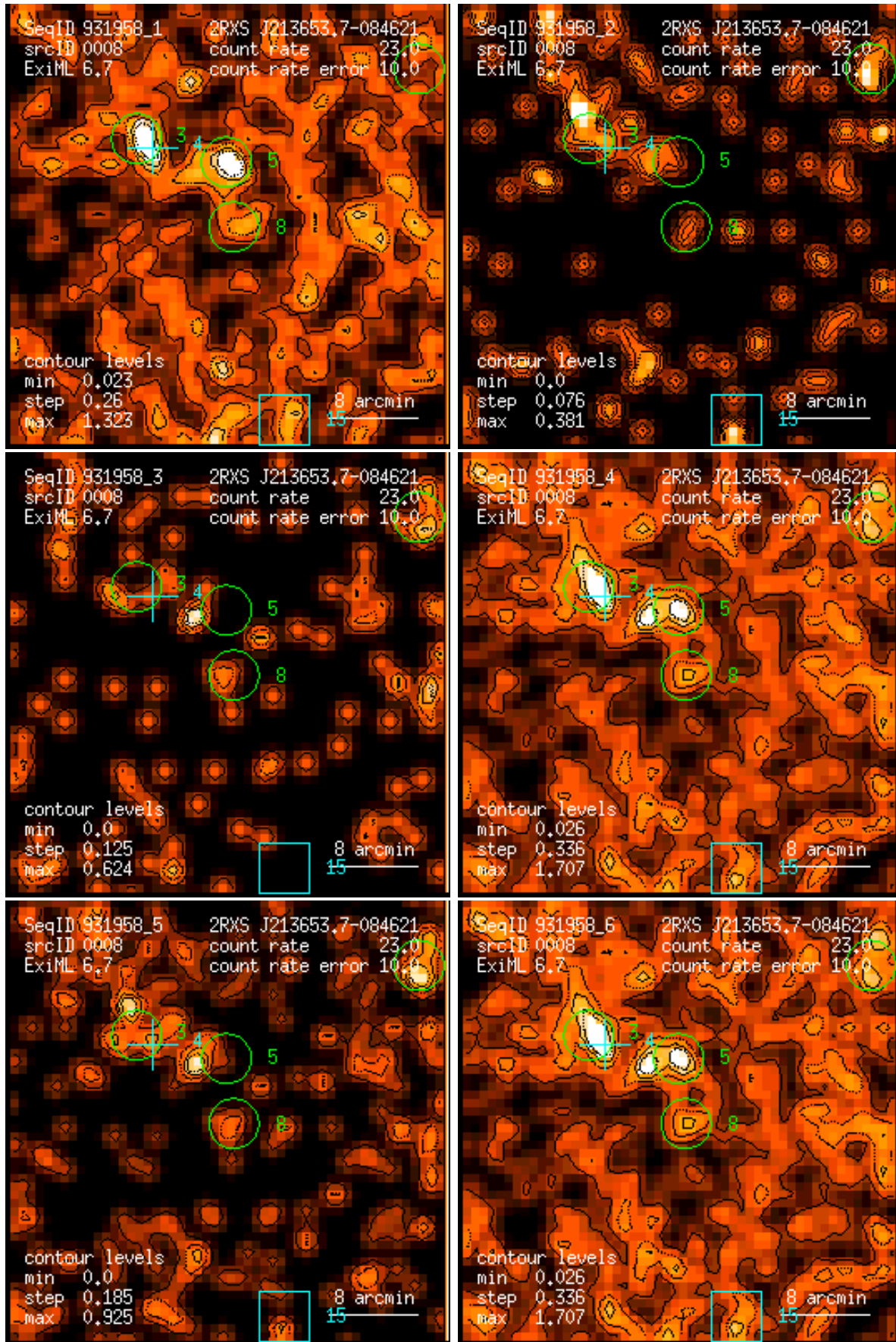
Figure 8: RASS 931958: detection 0008: band rate images, Gaussian filter: (1) PSPC channels 11 – 41, (2) 52 – 90, (3) 91 – 201, (4) 11 – 235, (5) 52 – 201, (6) 11 – 201. Broad band rates in counts/ks. Band rate contour levels in counts/ks/arcmin 2 .
