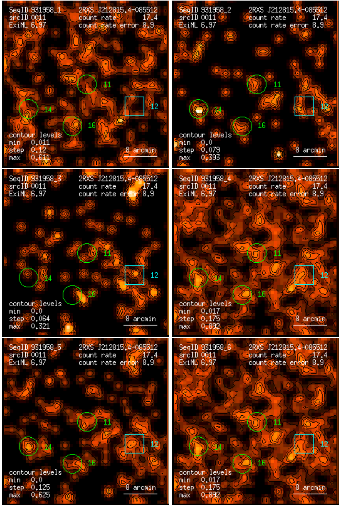
Figure 11: RASS 931958: detection 0011: band rate images, Gaussian filter: (1) PSPC channels 11 – 41, (2) 52 – 90, (3) 91 – 201, (4) 11 – 235, (5) 52 – 201, (6) 11 – 201. Broad band rates in counts/ks. Band rate contour levels in counts/ks/arcmin 2 .
