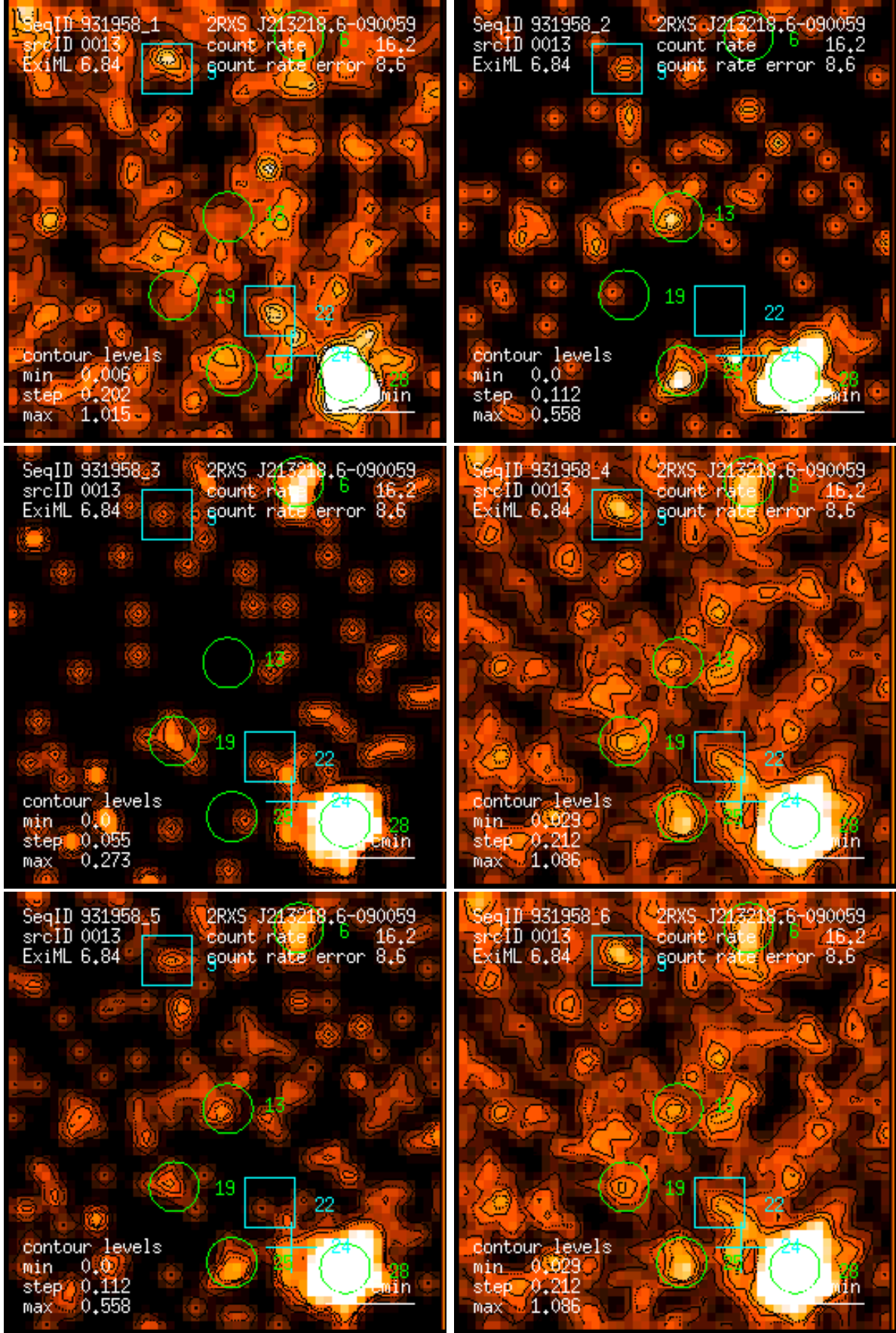
Figure 13: RASS 931958: detection 0013: band rate images, Gaussian filter: (1) PSPC channels 11 – 41, (2) 52 – 90, (3) 91 – 201, (4) 11 – 235, (5) 52 – 201, (6) 11 – 201. Broad band rates in counts/ks. Band rate contour levels in counts/ks/arcmin 2 .
