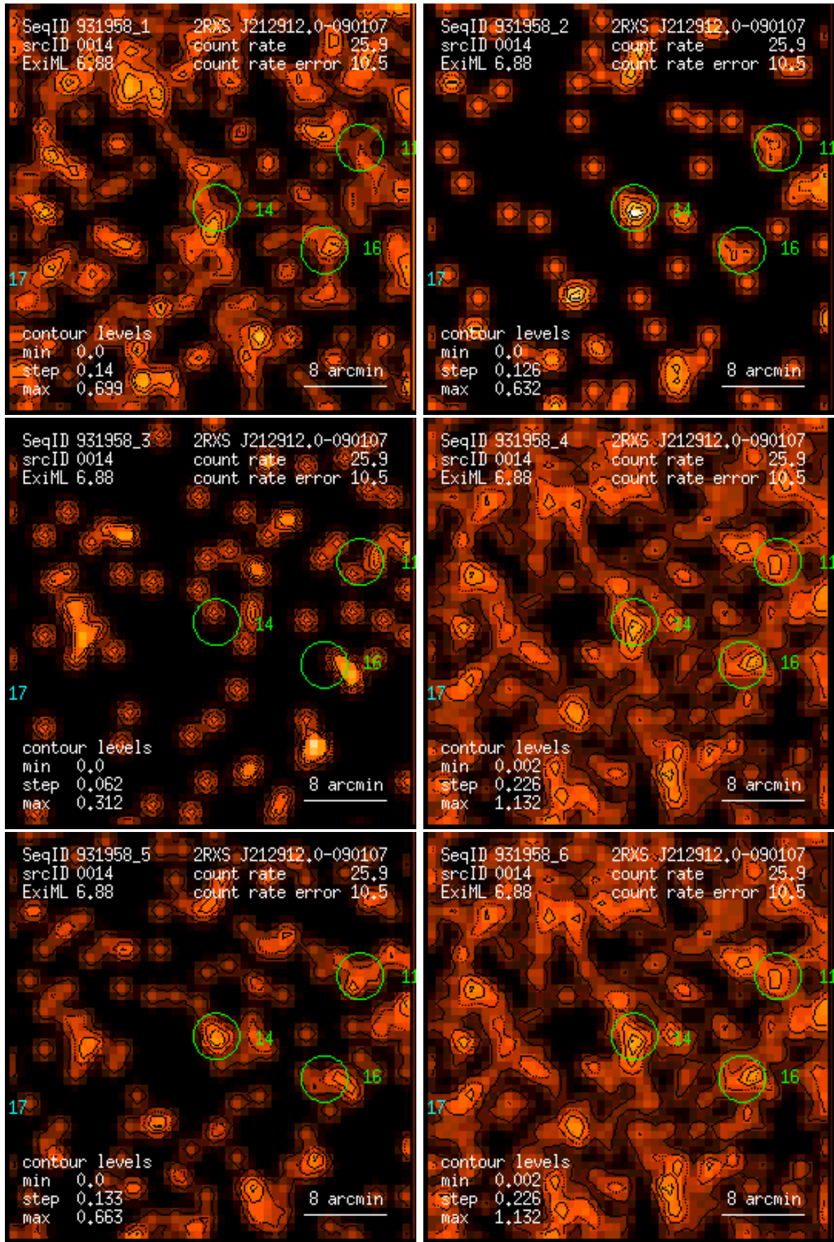
Figure 14: RASS 931958: detection 0014: band rate images, Gaussian filter: (1) PSPC channels 11 – 41, (2) 52 – 90, (3) 91 – 201, (4) 11 – 235, (5) 52 – 201, (6) 11 – 201. Broad band rates in counts/ks. Band rate contour levels in counts/ks/arcmin 2 .
