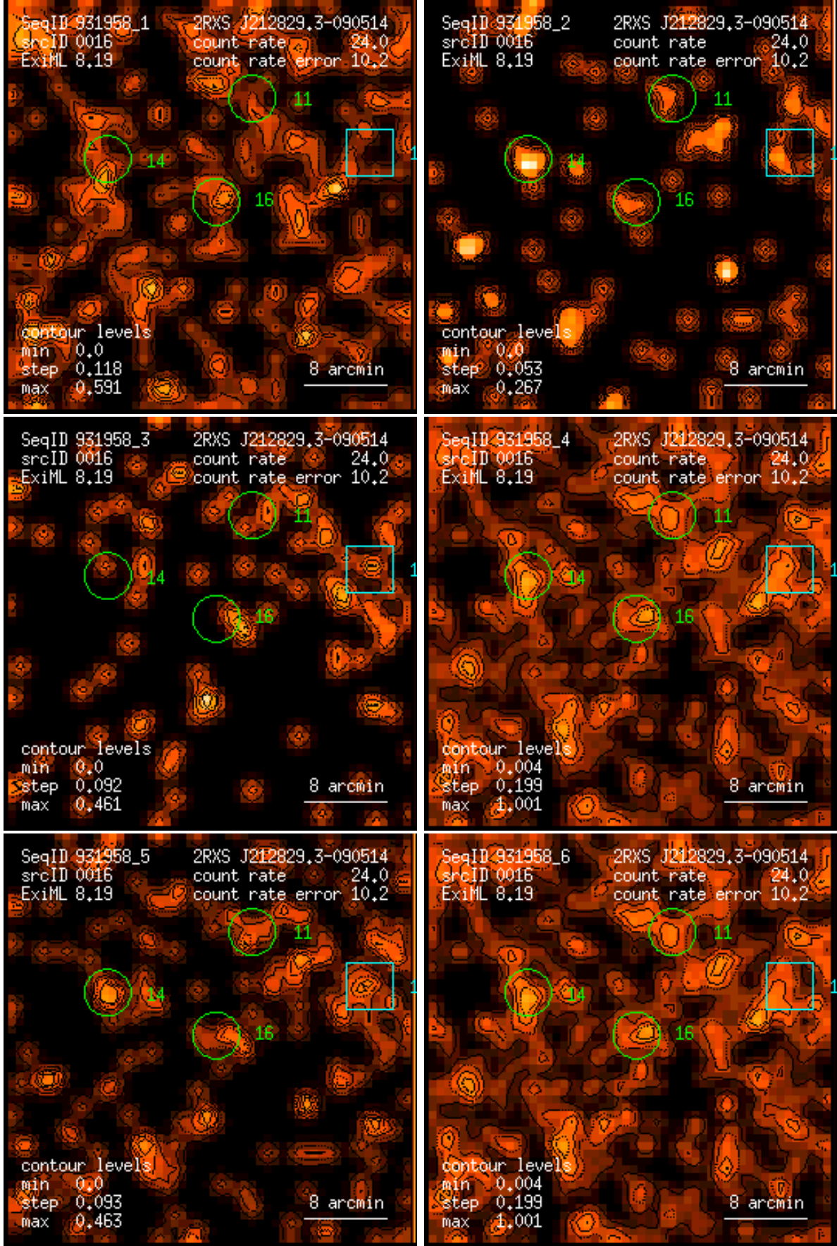
Figure 16: RASS 931958: detection 0016: band rate images, Gaussian filter: (1) PSPC channels 11 – 41, (2) 52 – 90, (3) 91 – 201, (4) 11 – 235, (5) 52 – 201, (6) 11 – 201. Broad band rates in counts/ks. Band rate contour levels in counts/ks/arcmin 2 .
