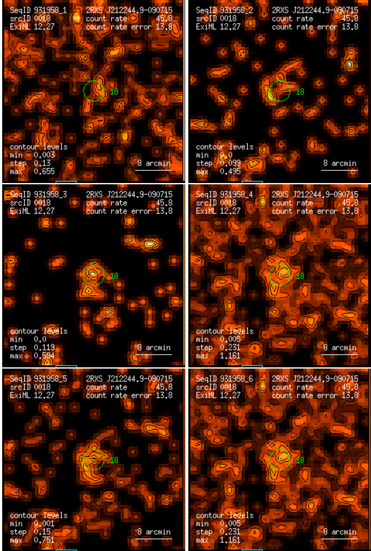
Figure 18: RASS 931958: detection 0018: band rate images, Gaussian filter: (1) PSPC channels 11 – 41, (2) 52 – 90, (3) 91 – 201, (4) 11 – 235, (5) 52 – 201, (6) 11 – 201. Broad band rates in counts/ks. Band rate contour levels in counts/ks/arcmin 2 .
