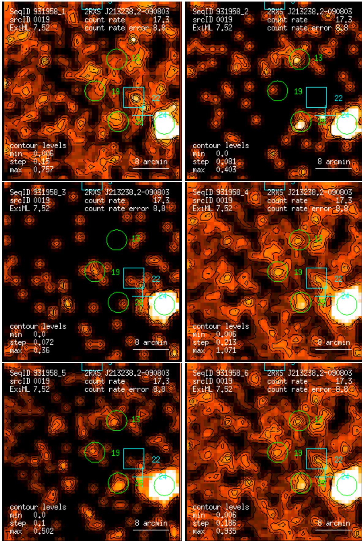
Figure 19: RASS 931958: detection 0019: band rate images, Gaussian filter: (1) PSPC channels 11 – 41, (2) 52 – 90, (3) 91 – 201, (4) 11 – 235, (5) 52 – 201, (6) 11 – 201. Broad band rates in counts/ks. Band rate contour levels in counts/ks/arcmin 2 .
