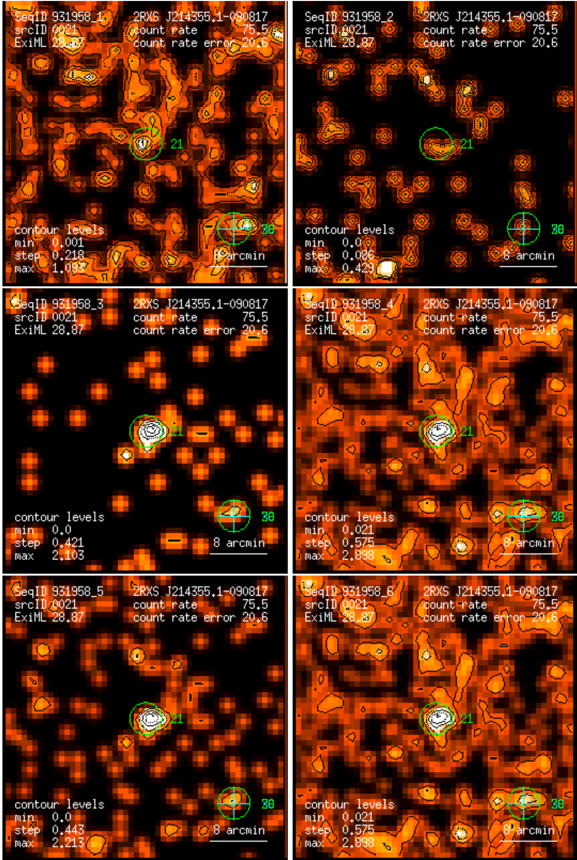
Figure 21: RASS 931958: detection 0021: band rate images, Gaussian filter: (1) PSPC channels 11 – 41, (2) 52 – 90, (3) 91 – 201, (4) 11 – 235, (5) 52 – 201, (6) 11 – 201. Broad band rates in counts/ks. Band rate contour levels in counts/ks/arcmin 2 .
