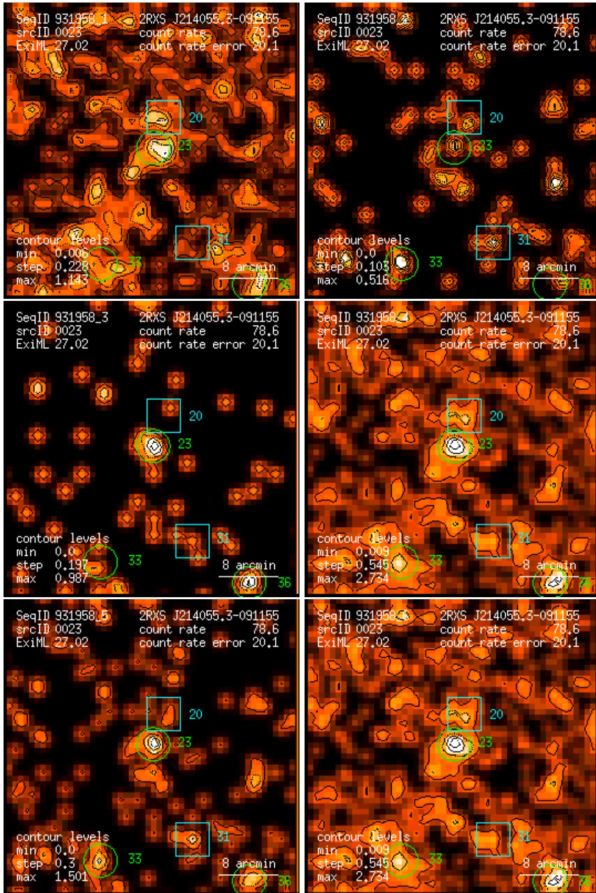
Figure 23: RASS 931958: detection 0023: band rate images, Gaussian filter: (1) PSPC channels 11 – 41, (2) 52 – 90, (3) 91 – 201, (4) 11 – 235, (5) 52 – 201, (6) 11 – 201. Broad band rates in counts/ks. Band rate contour levels in counts/ks/arcmin 2 .
