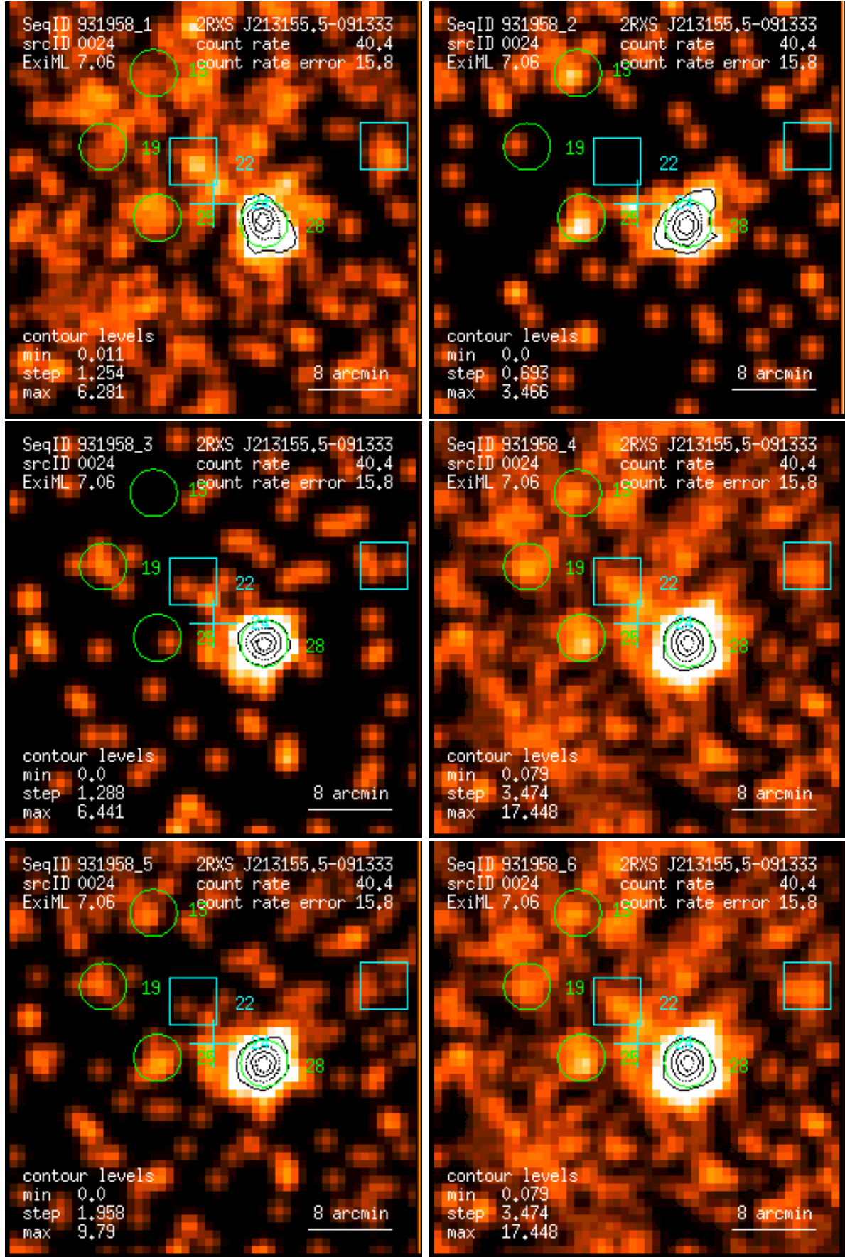
Figure 24: RASS 931958: detection 0024: band rate images, Gaussian filter: (1) PSPC channels 11 – 41, (2) 52 – 90, (3) 91 – 201, (4) 11 – 235, (5) 52 – 201, (6) 11 – 201. Broad band rates in counts/ks. Band rate contour levels in counts/ks/arcmin 2 .
