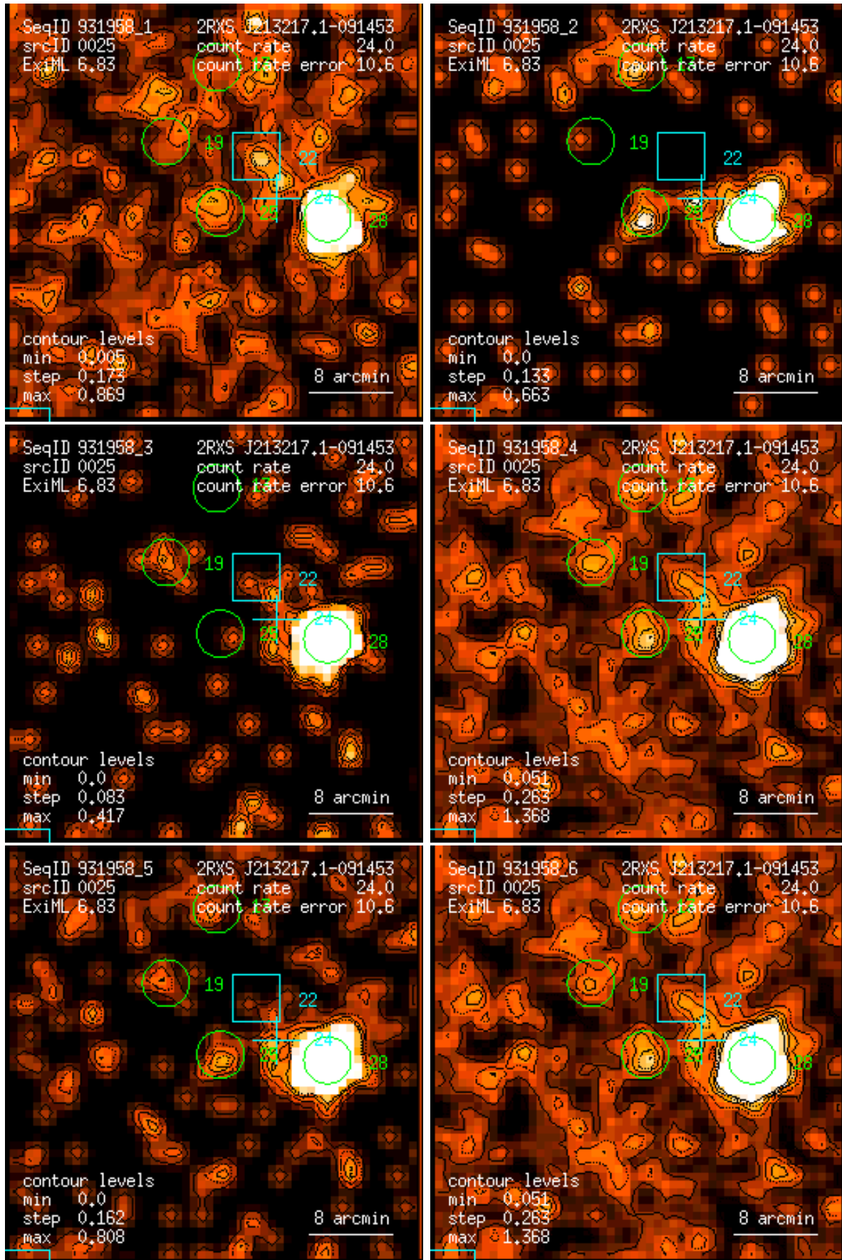
Figure 25: RASS 931958: detection 0025: band rate images, Gaussian filter: (1) PSPC channels 11 – 41, (2) 52 – 90, (3) 91 – 201, (4) 11 – 235, (5) 52 – 201, (6) 11 – 201. Broad band rates in counts/ks. Band rate contour levels in counts/ks/arcmin 2 .
