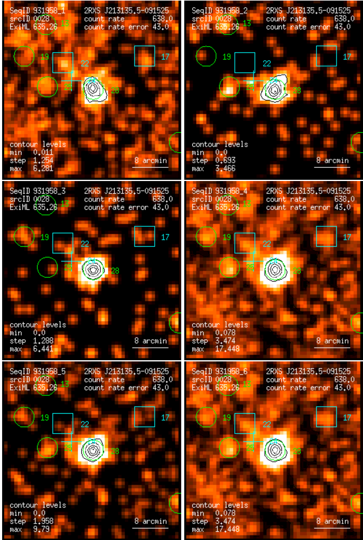
Figure 28: RASS 931958: detection 0028: band rate images, Gaussian filter: (1) PSPC channels 11 – 41, (2) 52 – 90, (3) 91 – 201, (4) 11 – 235, (5) 52 – 201, (6) 11 – 201. Broad band rates in counts/ks. Band rate contour levels in counts/ks/arcmin 2 .
