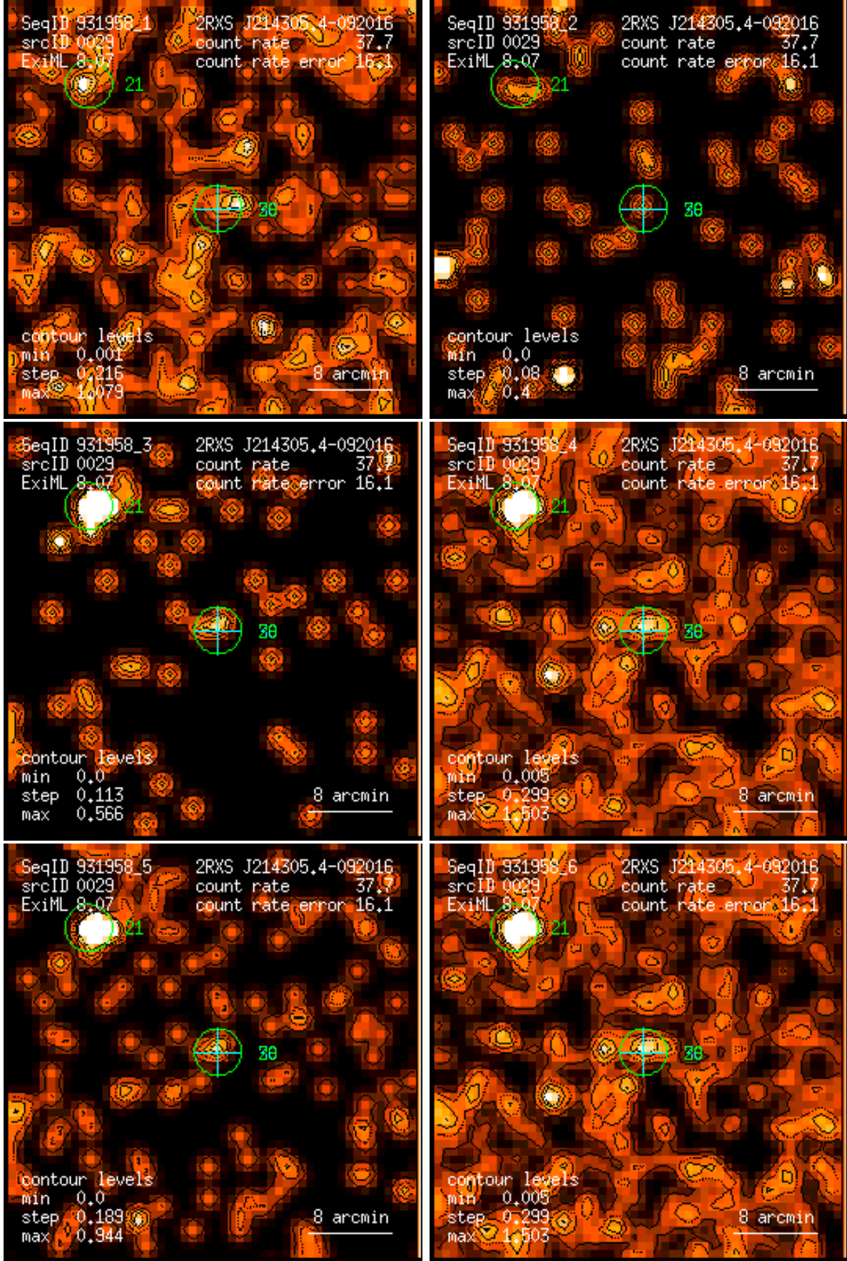
Figure 29: RASS 931958: detection 0029: band rate images, Gaussian filter: (1) PSPC channels 11 – 41, (2) 52 – 90, (3) 91 – 201, (4) 11 – 235, (5) 52 – 201, (6) 11 – 201. Broad band rates in counts/ks. Band rate contour levels in counts/ks/arcmin 2 .
