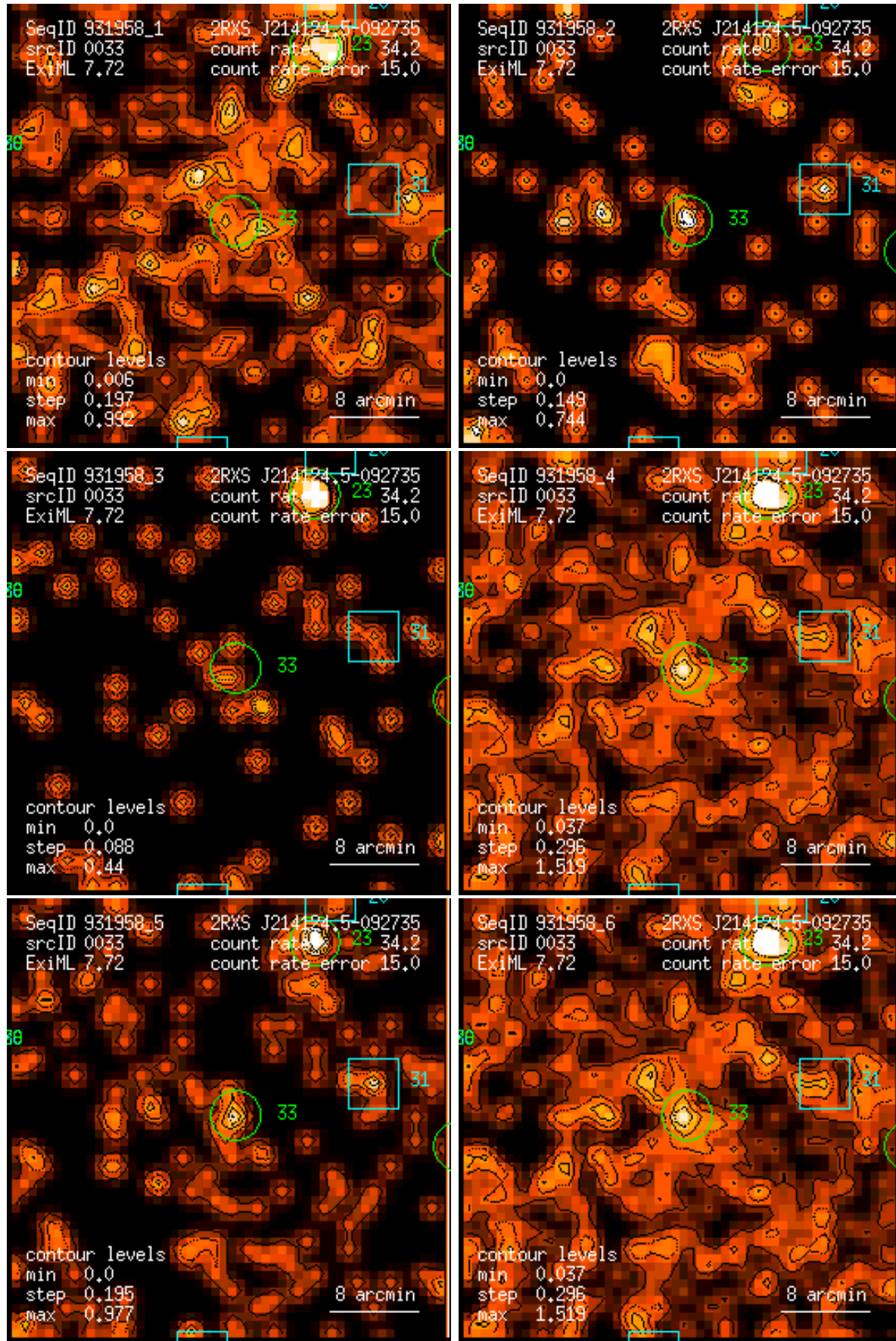
Figure 33: RASS 931958: detection 0033: band rate images, Gaussian filter: (1) PSPC channels 11 – 41, (2) 52 – 90, (3) 91 – 201, (4) 11 – 235, (5) 52 – 201, (6) 11 – 201. Broad band rates in counts/ks. Band rate contour levels in counts/ks/arcmin 2 .
