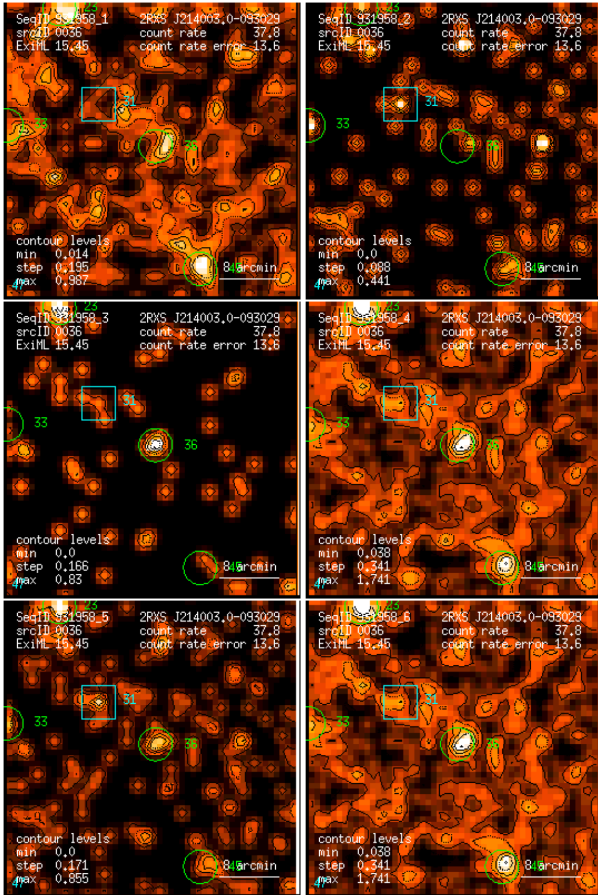
Figure 36: RASS 931958: detection 0036: band rate images, Gaussian filter: (1) PSPC channels 11 – 41, (2) 52 – 90, (3) 91 – 201, (4) 11 – 235, (5) 52 – 201, (6) 11 – 201. Broad band rates in counts/ks. Band rate contour levels in counts/ks/arcmin 2 .
