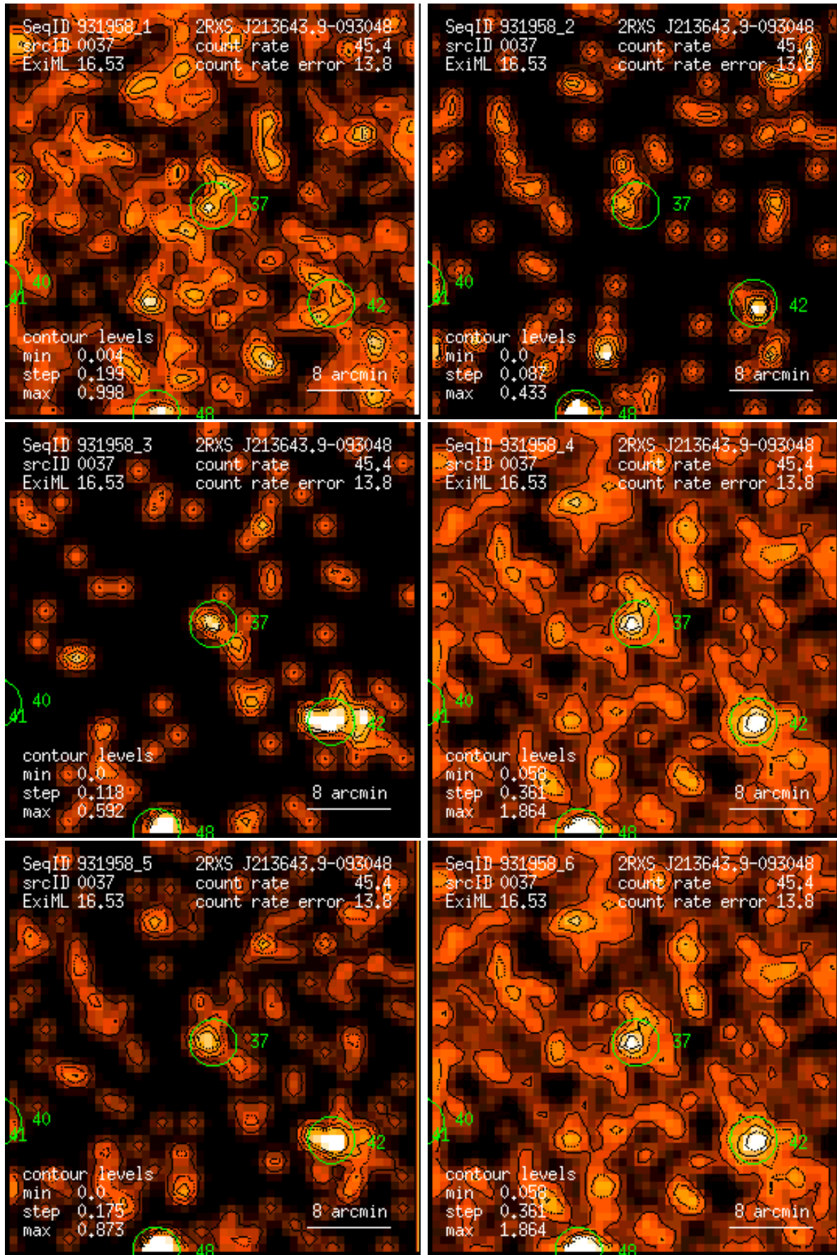
Figure 37: RASS 931958: detection 0037: band rate images, Gaussian filter: (1) PSPC channels 11 – 41, (2) 52 – 90, (3) 91 – 201, (4) 11 – 235, (5) 52 – 201, (6) 11 – 201. Broad band rates in counts/ks. Band rate contour levels in counts/ks/arcmin 2 .
