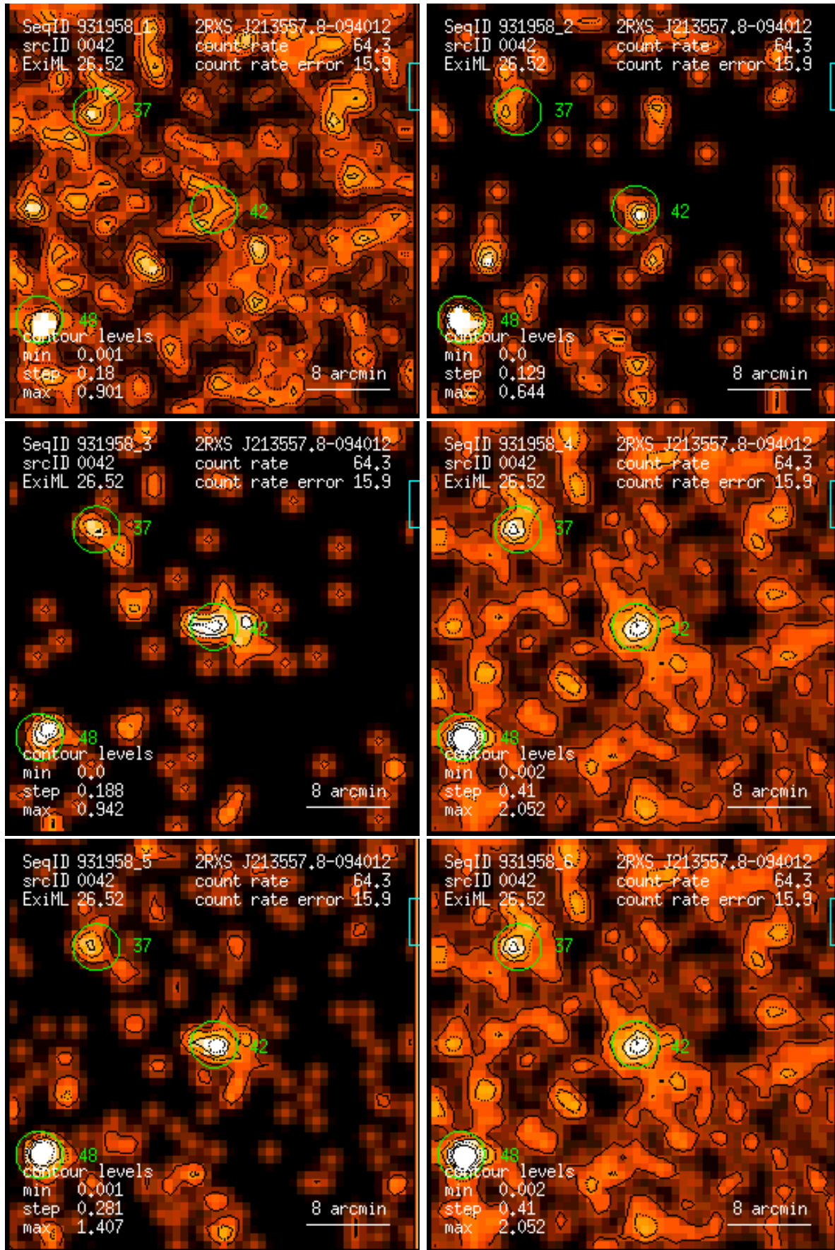
Figure 42: RASS 931958: detection 0042: band rate images, Gaussian filter: (1) PSPC channels 11 – 41, (2) 52 – 90, (3) 91 – 201, (4) 11 – 235, (5) 52 – 201, (6) 11 – 201. Broad band rates in counts/ks. Band rate contour levels in counts/ks/arcmin 2 .
