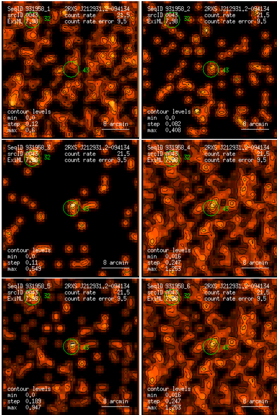
Figure 43: RASS 931958: detection 0043: band rate images, Gaussian filter: (1) PSPC channels 11 – 41, (2) 52 – 90, (3) 91 – 201, (4) 11 – 235, (5) 52 – 201, (6) 11 – 201. Broad band rates in counts/ks. Band rate contour levels in counts/ks/arcmin 2 .
