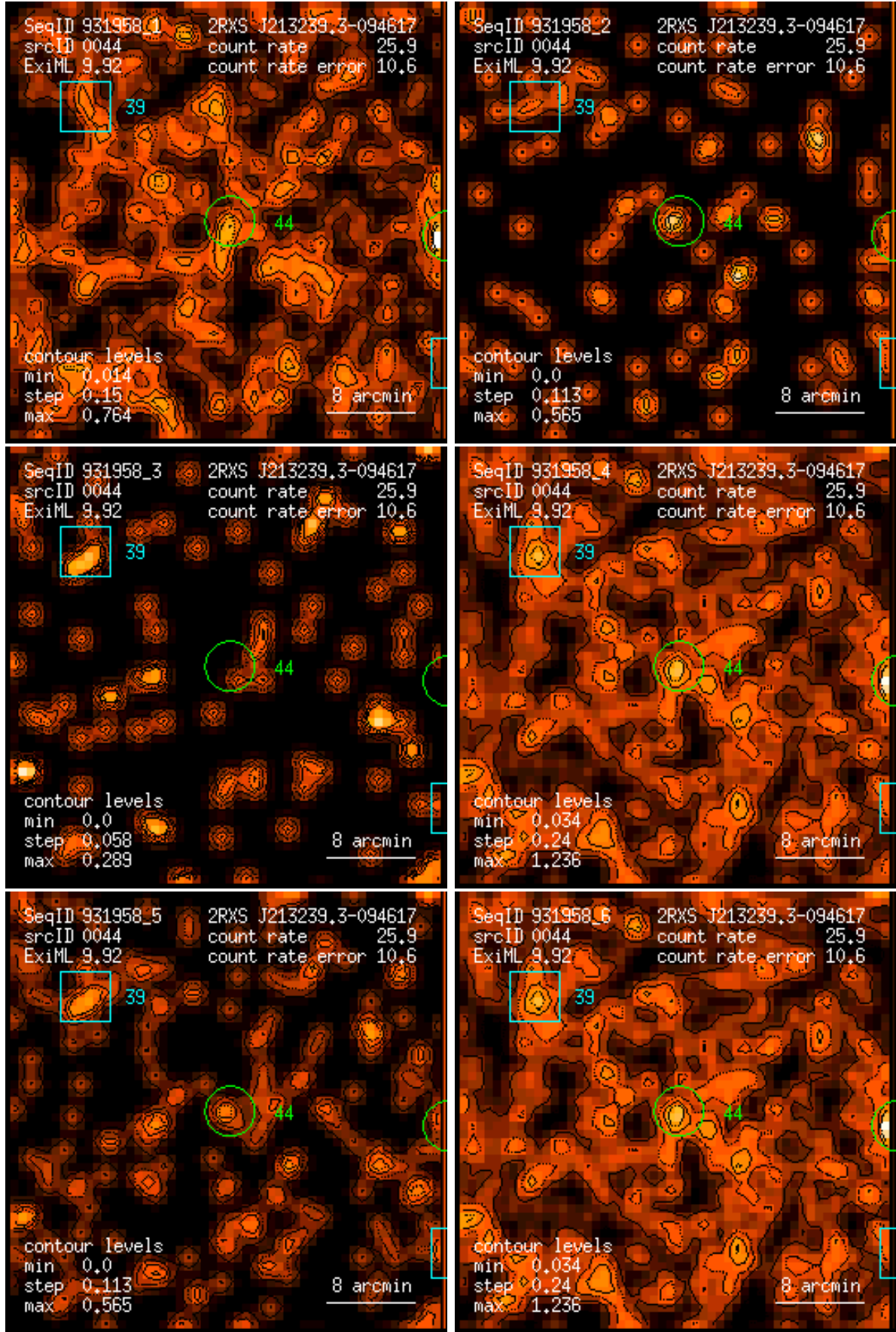
Figure 44: RASS 931958: detection 0044: band rate images, Gaussian filter: (1) PSPC channels 11 – 41, (2) 52 – 90, (3) 91 – 201, (4) 11 – 235, (5) 52 – 201, (6) 11 – 201. Broad band rates in counts/ks. Band rate contour levels in counts/ks/arcmin 2 .
