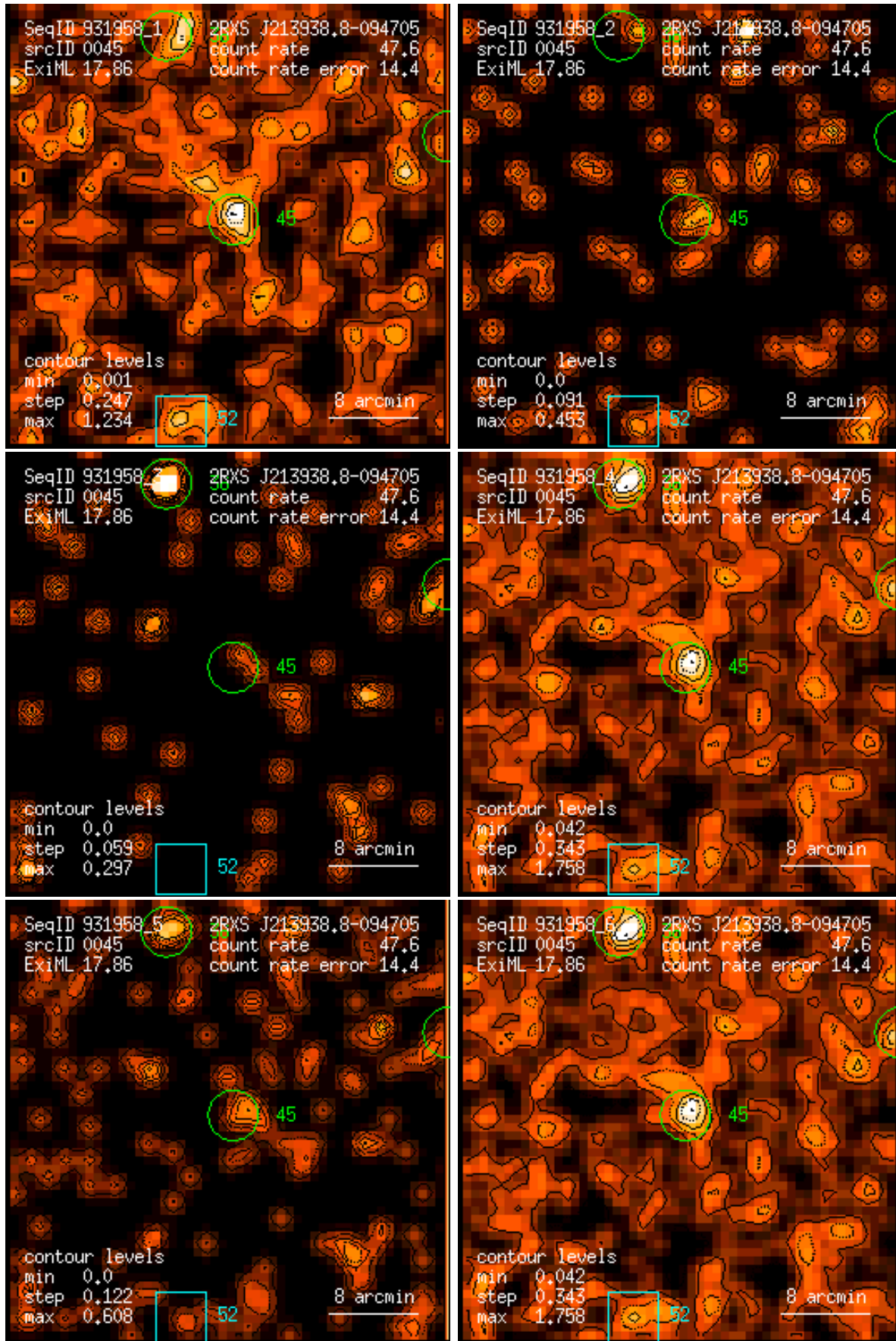
Figure 45: RASS 931958: detection 0045: band rate images, Gaussian filter: (1) PSPC channels 11 – 41, (2) 52 – 90, (3) 91 – 201, (4) 11 – 235, (5) 52 – 201, (6) 11 – 201. Broad band rates in counts/ks. Band rate contour levels in counts/ks/arcmin 2 .
