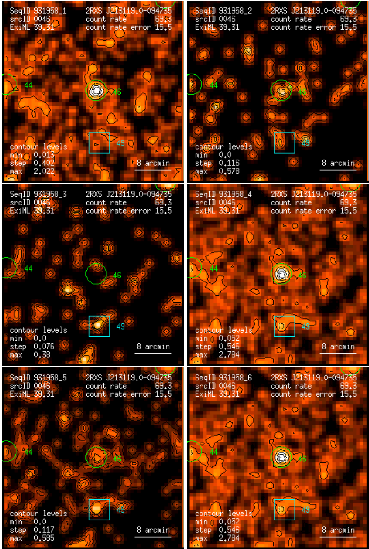
Figure 46: RASS 931958: detection 0046: band rate images, Gaussian filter: (1) PSPC channels 11 – 41, (2) 52 – 90, (3) 91 – 201, (4) 11 – 235, (5) 52 – 201, (6) 11 – 201. Broad band rates in counts/ks. Band rate contour levels in counts/ks/arcmin 2 .
