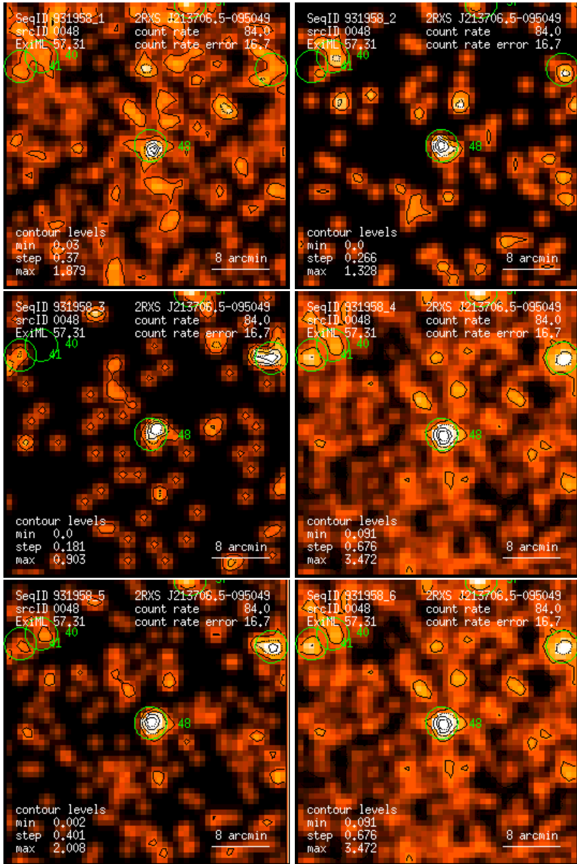
Figure 48: RASS 931958: detection 0048: band rate images, Gaussian filter: (1) PSPC channels 11 – 41, (2) 52 – 90, (3) 91 – 201, (4) 11 – 235, (5) 52 – 201, (6) 11 – 201. Broad band rates in counts/ks. Band rate contour levels in counts/ks/arcmin 2 .
