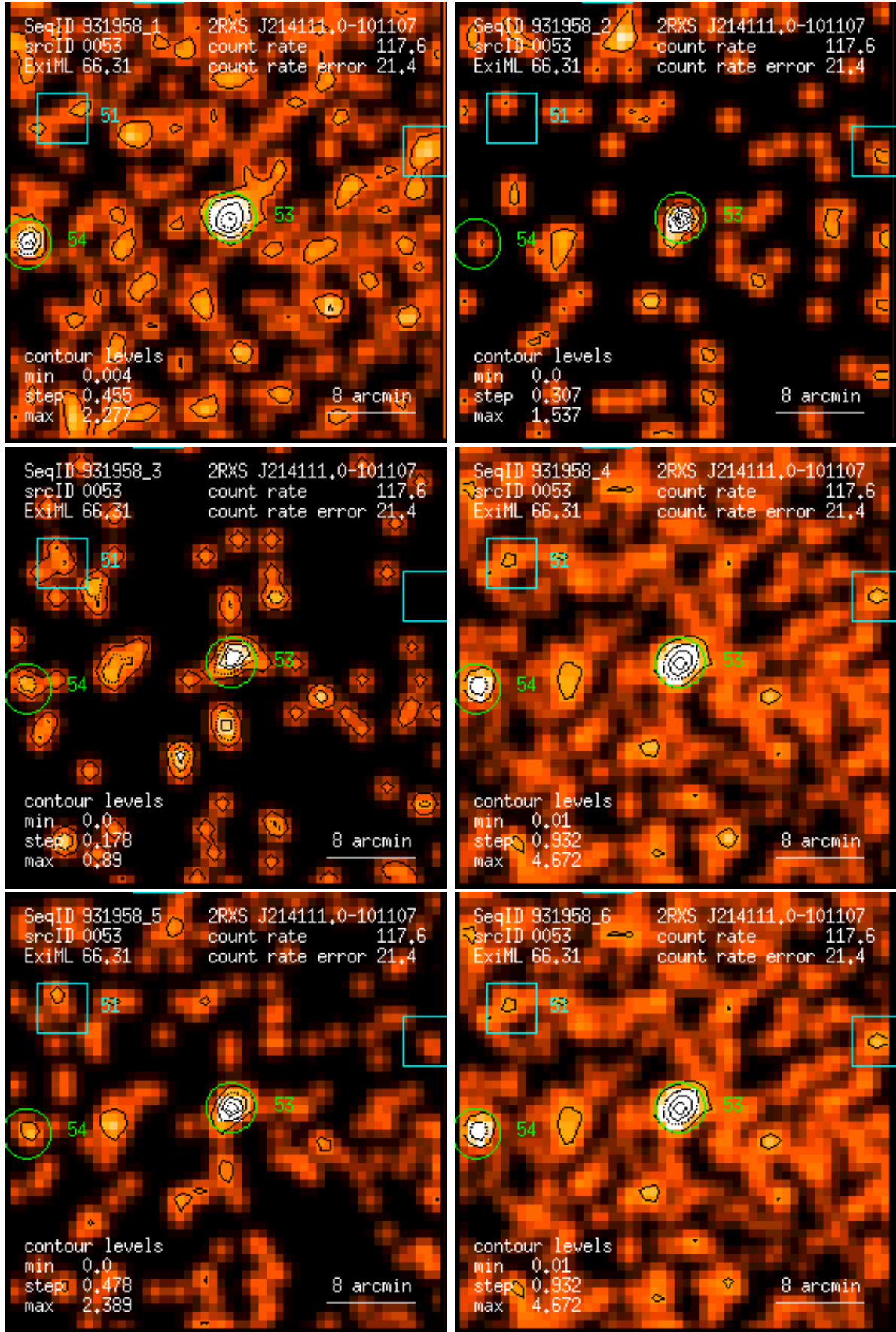
Figure 53: RASS 931958: detection 0053: band rate images, Gaussian filter: (1) PSPC channels 11 – 41, (2) 52 – 90, (3) 91 – 201, (4) 11 – 235, (5) 52 – 201, (6) 11 – 201. Broad band rates in counts/ks. Band rate contour levels in counts/ks/arcmin 2 .
