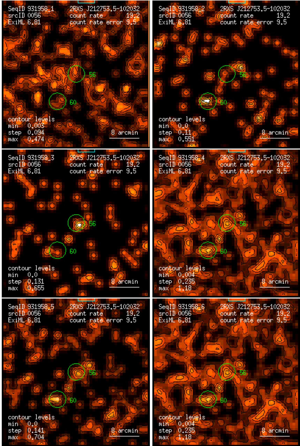
Figure 56: RASS 931958: detection 0056: band rate images, Gaussian filter: (1) PSPC channels 11 – 41, (2) 52 – 90, (3) 91 – 201, (4) 11 – 235, (5) 52 – 201, (6) 11 – 201. Broad band rates in counts/ks. Band rate contour levels in counts/ks/arcmin 2 .
