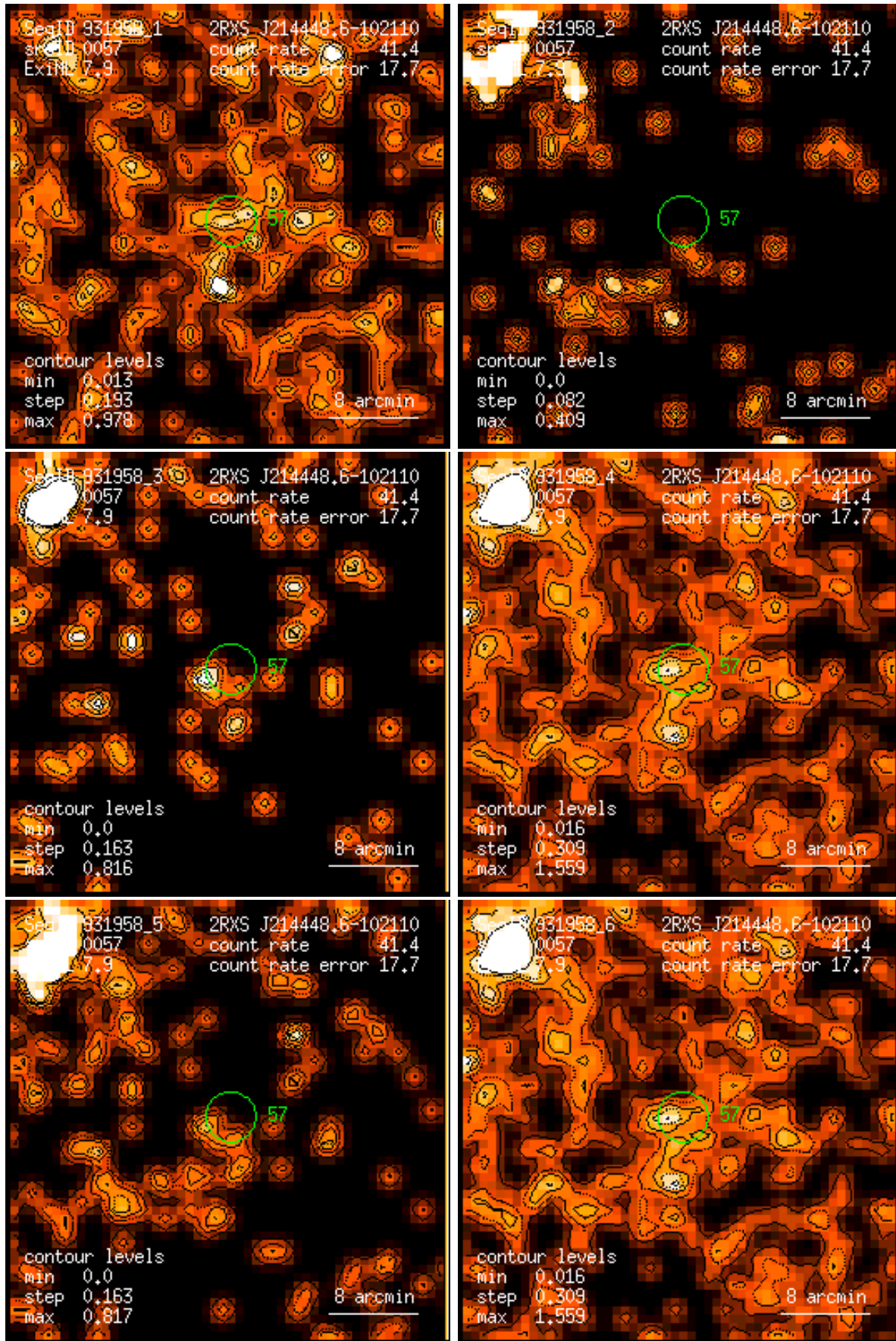
Figure 57: RASS 931958: detection 0057: band rate images, Gaussian filter: (1) PSPC channels 11 – 41, (2) 52 – 90, (3) 91 – 201, (4) 11 – 235, (5) 52 – 201, (6) 11 – 201. Broad band rates in counts/ks. Band rate contour levels in counts/ks/arcmin 2 .
