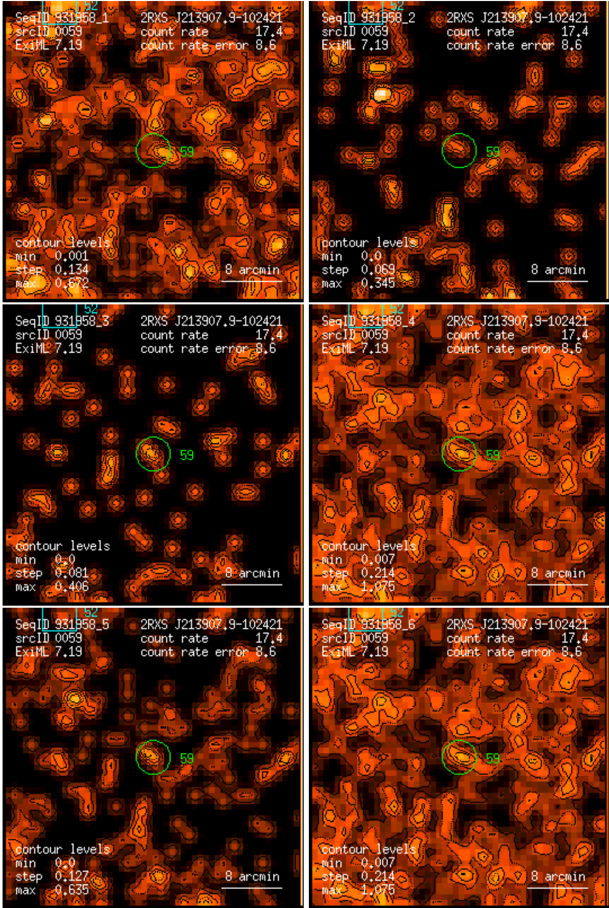
Figure 59: RASS 931958: detection 0059: band rate images, Gaussian filter: (1) PSPC channels 11 – 41, (2) 52 – 90, (3) 91 – 201, (4) 11 – 235, (5) 52 – 201, (6) 11 – 201. Broad band rates in counts/ks. Band rate contour levels in counts/ks/arcmin 2 .
