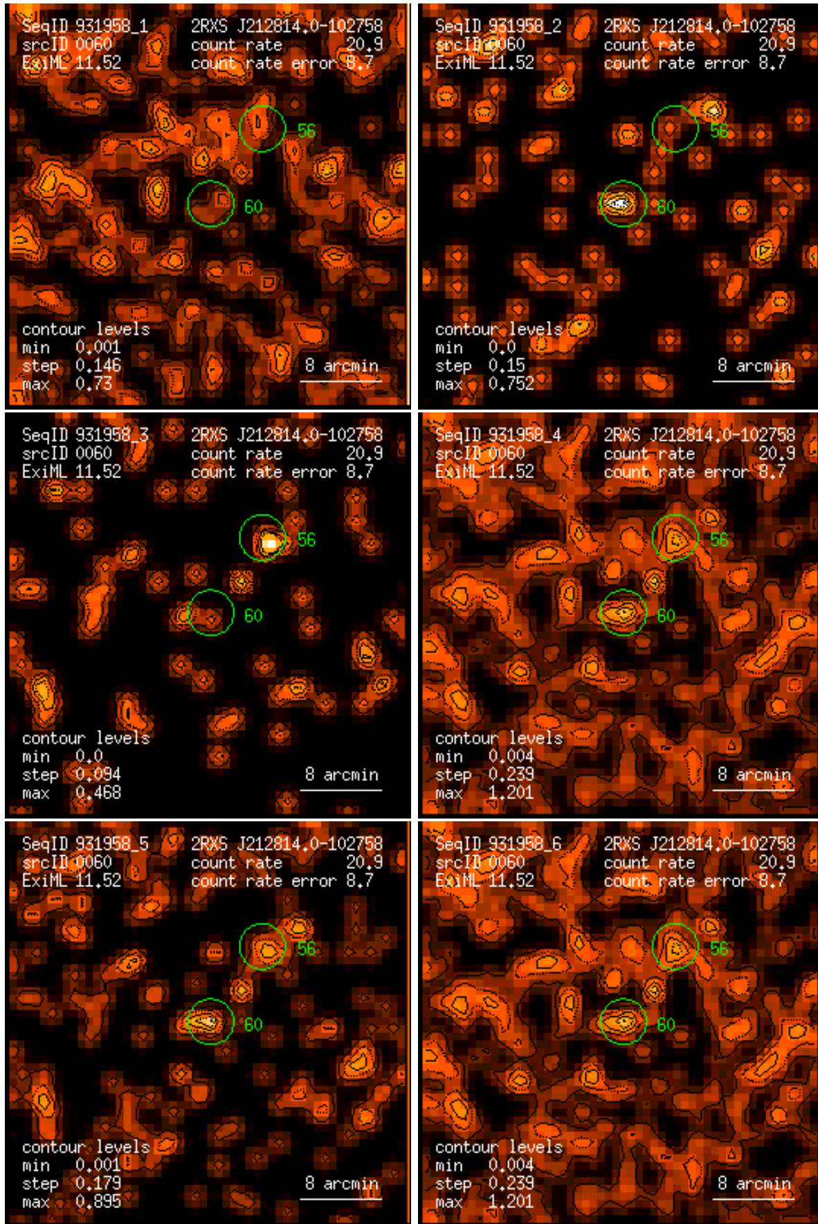
Figure 60: RASS 931958: detection 0060: band rate images, Gaussian filter: (1) PSPC channels 11 – 41, (2) 52 – 90, (3) 91 – 201, (4) 11 – 235, (5) 52 – 201, (6) 11 – 201. Broad band rates in counts/ks. Band rate contour levels in counts/ks/arcmin 2 .
