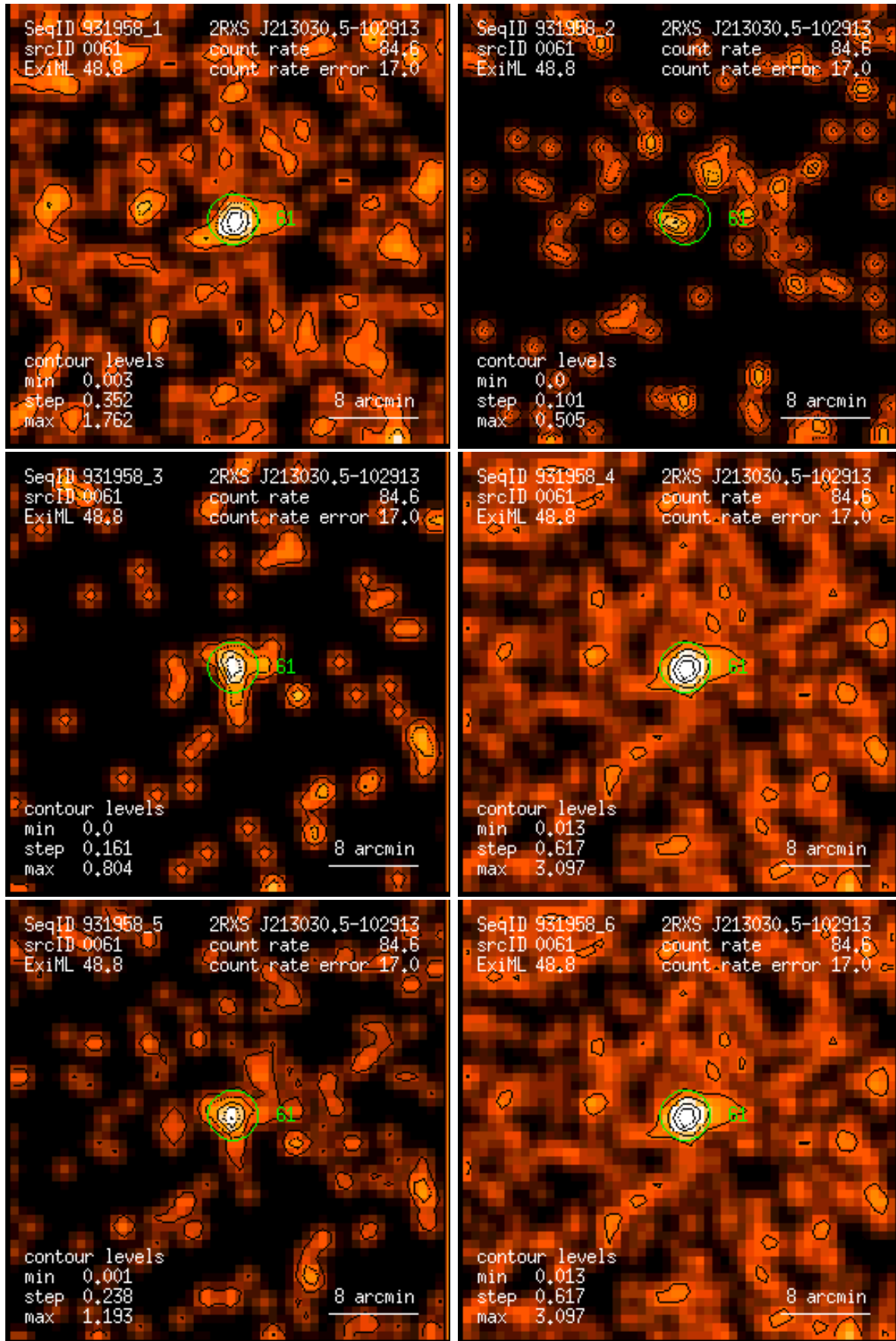
Figure 61: RASS 931958: detection 0061: band rate images, Gaussian filter: (1) PSPC channels 11 – 41, (2) 52 – 90, (3) 91 – 201, (4) 11 – 235, (5) 52 – 201, (6) 11 – 201. Broad band rates in counts/ks. Band rate contour levels in counts/ks/arcmin 2 .
