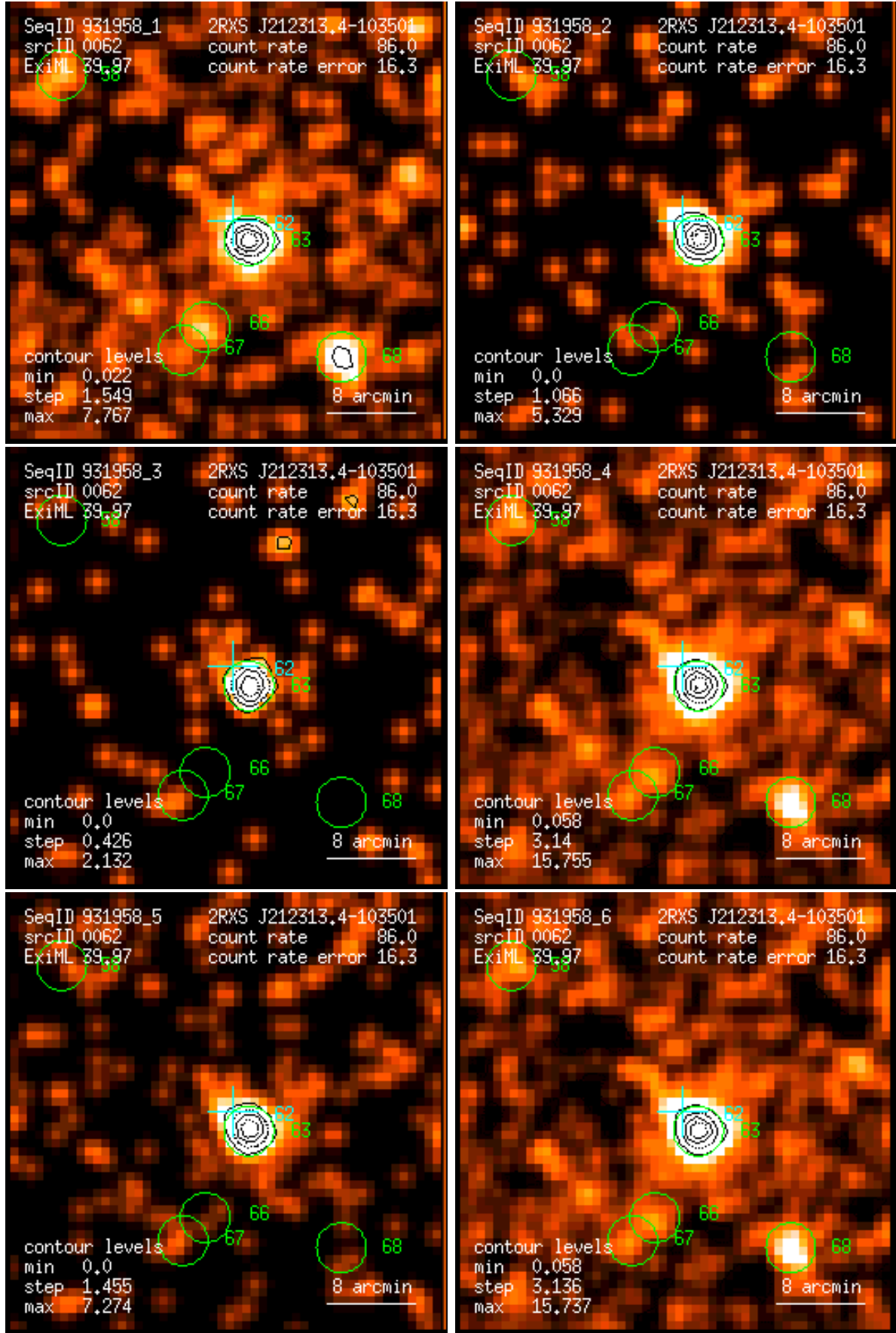
Figure 62: RASS 931958: detection 0062: band rate images, Gaussian filter: (1) PSPC channels 11 – 41, (2) 52 – 90, (3) 91 – 201, (4) 11 – 235, (5) 52 – 201, (6) 11 – 201. Broad band rates in counts/ks. Band rate contour levels in counts/ks/arcmin 2 .
