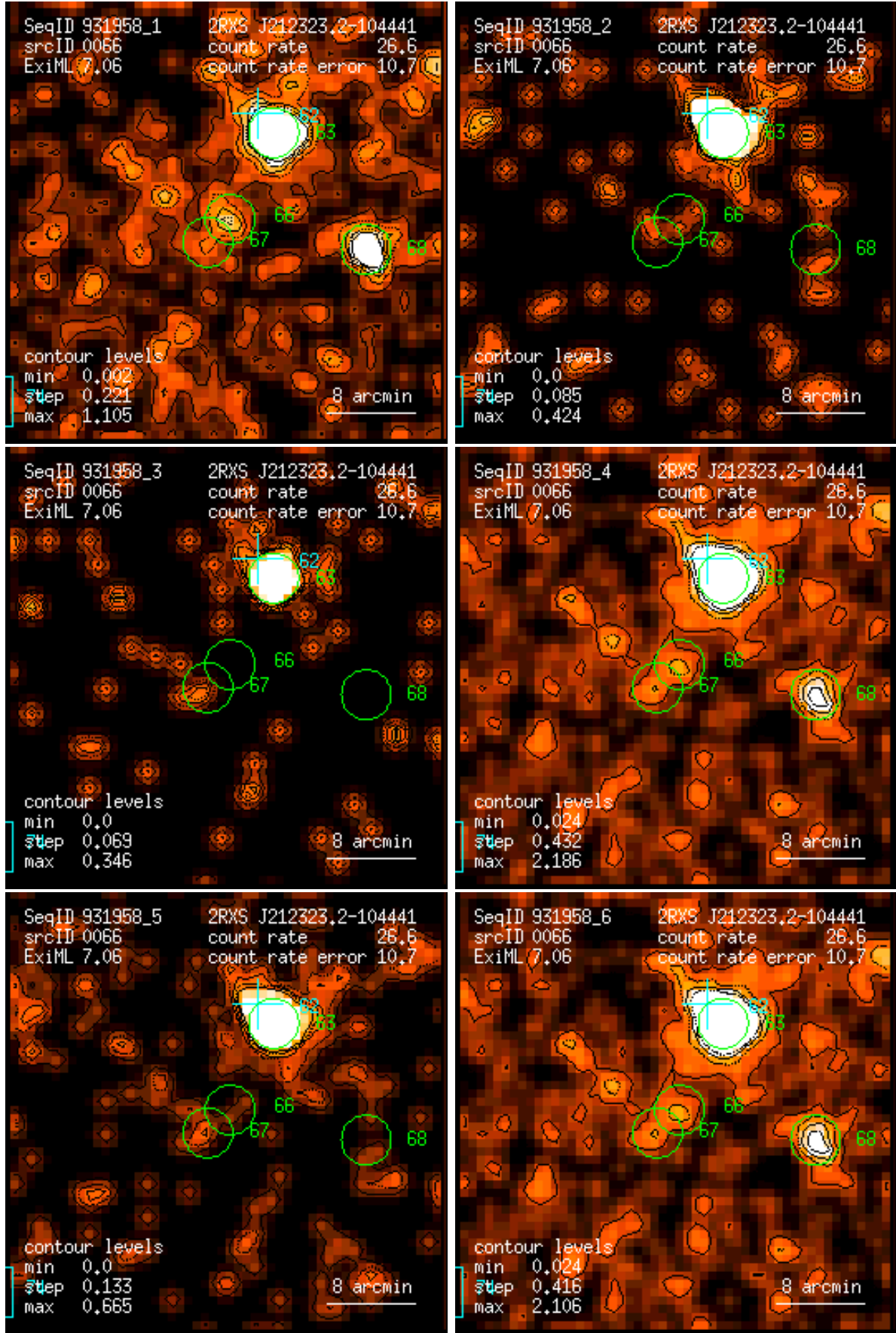
Figure 66: RASS 931958: detection 0066: band rate images, Gaussian filter: (1) PSPC channels 11 – 41, (2) 52 – 90, (3) 91 – 201, (4) 11 – 235, (5) 52 – 201, (6) 11 – 201. Broad band rates in counts/ks. Band rate contour levels in counts/ks/arcmin 2 .
