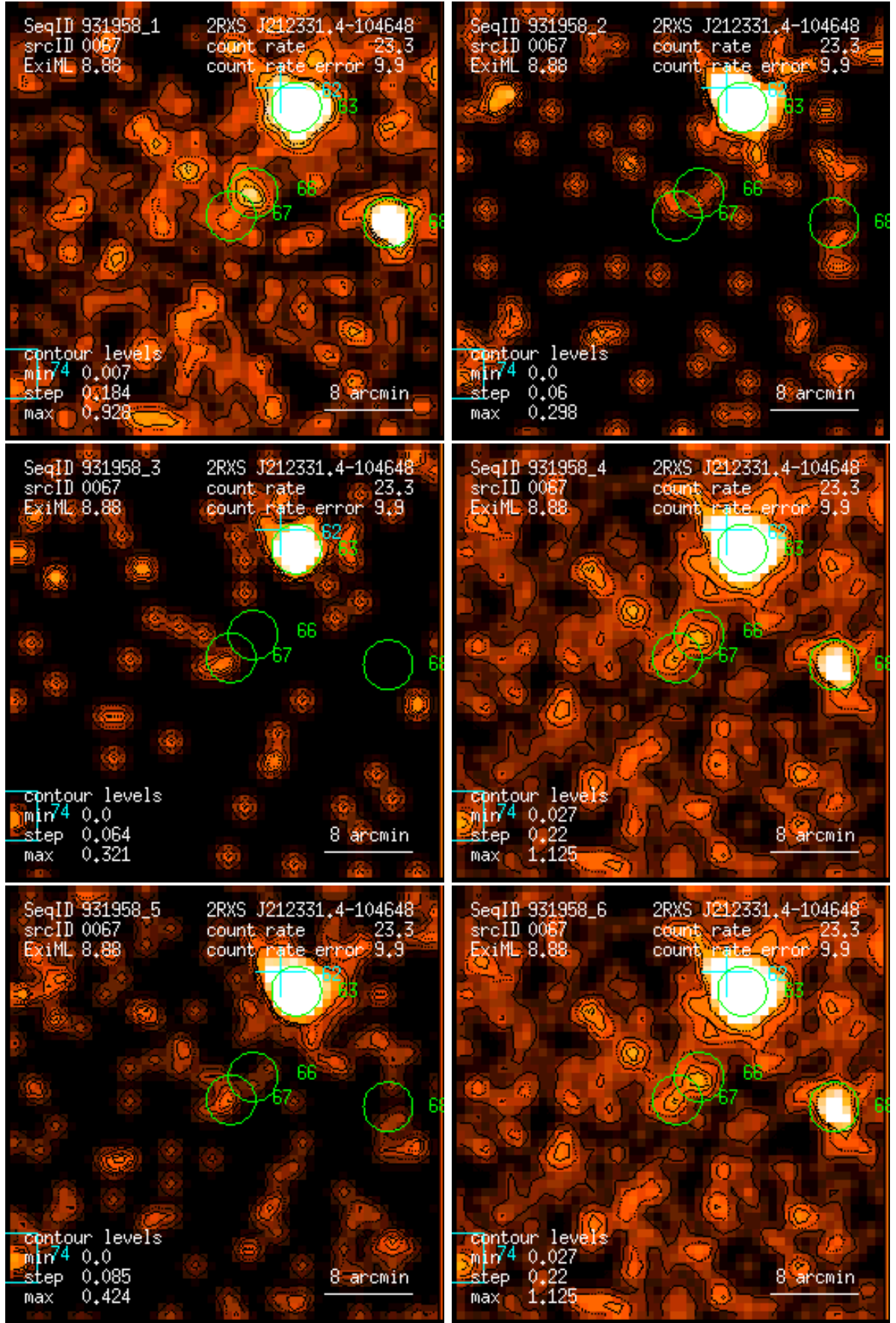
Figure 67: RASS 931958: detection 0067: band rate images, Gaussian filter: (1) PSPC channels 11 – 41, (2) 52 – 90, (3) 91 – 201, (4) 11 – 235, (5) 52 – 201, (6) 11 – 201. Broad band rates in counts/ks. Band rate contour levels in counts/ks/arcmin 2 .
