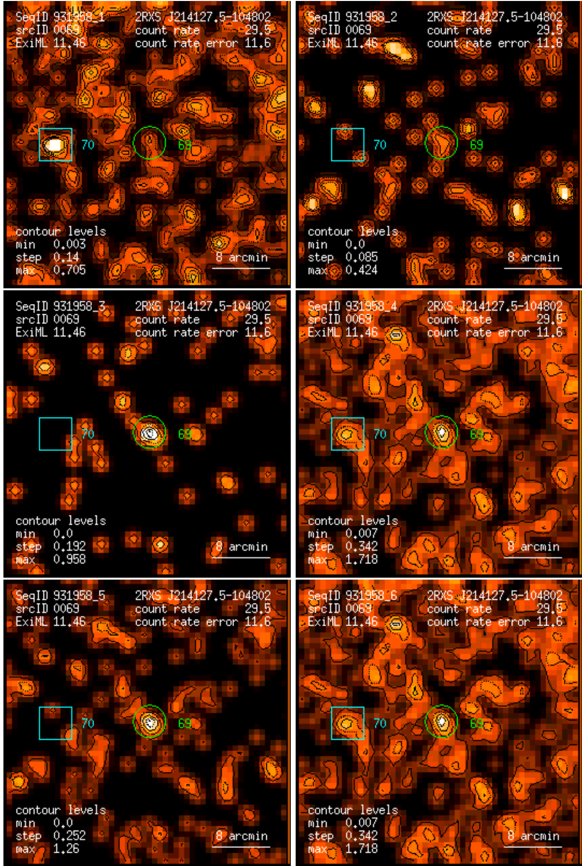
Figure 69: RASS 931958: detection 0069: band rate images, Gaussian filter: (1) PSPC channels 11 – 41, (2) 52 – 90, (3) 91 – 201, (4) 11 – 235, (5) 52 – 201, (6) 11 – 201. Broad band rates in counts/ks. Band rate contour levels in counts/ks/arcmin 2 .
