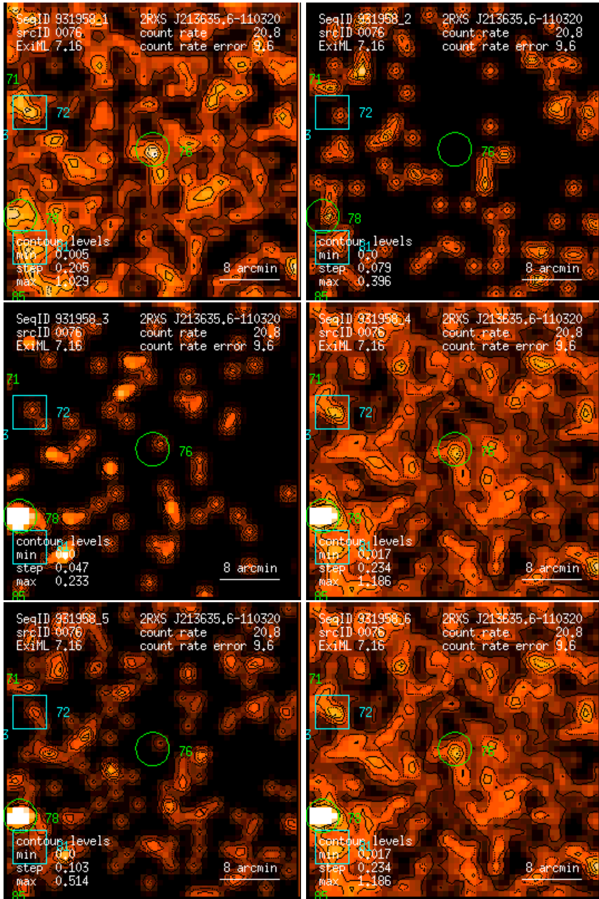
Figure 76: RASS 931958: detection 0076: band rate images, Gaussian filter: (1) PSPC channels 11 – 41, (2) 52 – 90, (3) 91 – 201, (4) 11 – 235, (5) 52 – 201, (6) 11 – 201. Broad band rates in counts/ks. Band rate contour levels in counts/ks/arcmin 2 .
