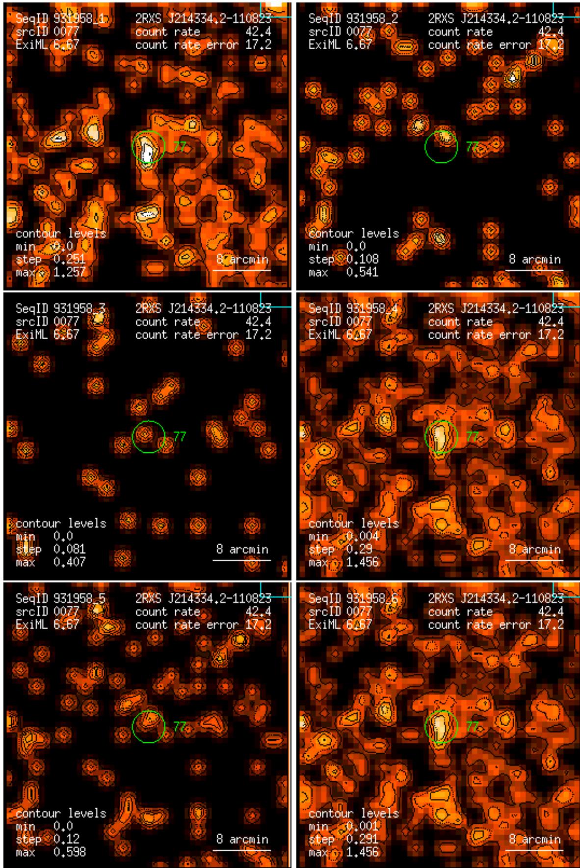
Figure 77: RASS 931958: detection 0077: band rate images, Gaussian filter: (1) PSPC channels 11 – 41, (2) 52 – 90, (3) 91 – 201, (4) 11 – 235, (5) 52 – 201, (6) 11 – 201. Broad band rates in counts/ks. Band rate contour levels in counts/ks/arcmin 2 .
