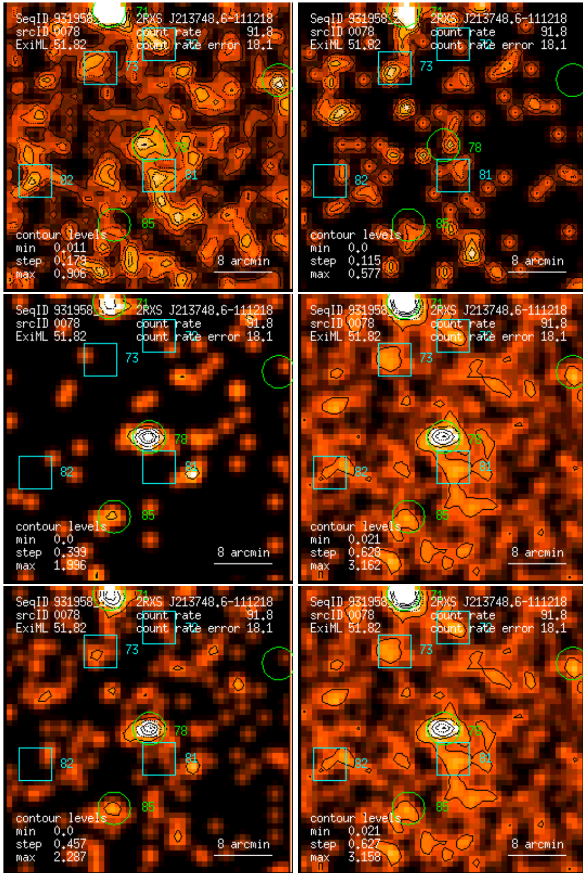
Figure 78: RASS 931958: detection 0078: band rate images, Gaussian filter: (1) PSPC channels 11 – 41, (2) 52 – 90, (3) 91 – 201, (4) 11 – 235, (5) 52 – 201, (6) 11 – 201. Broad band rates in counts/ks. Band rate contour levels in counts/ks/arcmin 2 .
