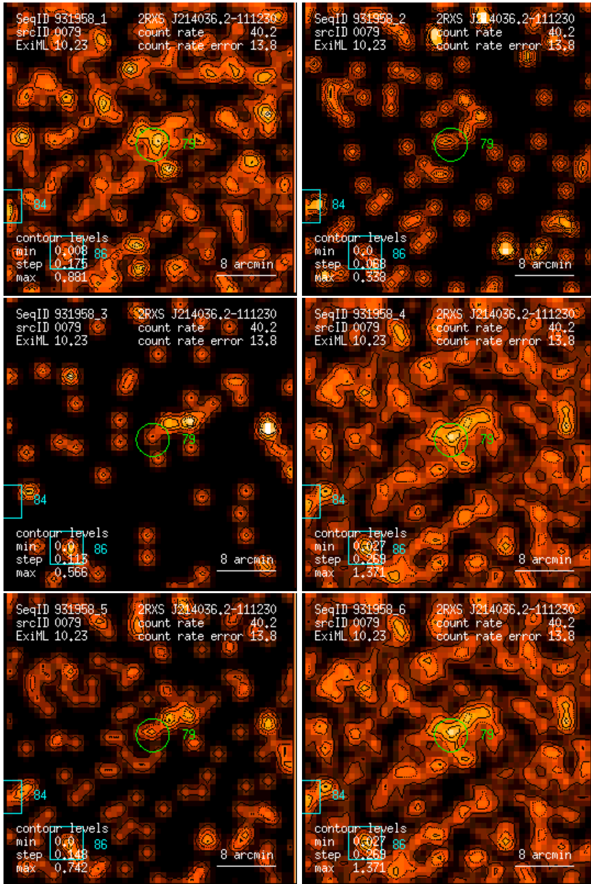
Figure 79: RASS 931958: detection 0079: band rate images, Gaussian filter: (1) PSPC channels 11 – 41, (2) 52 – 90, (3) 91 – 201, (4) 11 – 235, (5) 52 – 201, (6) 11 – 201. Broad band rates in counts/ks. Band rate contour levels in counts/ks/arcmin 2 .
