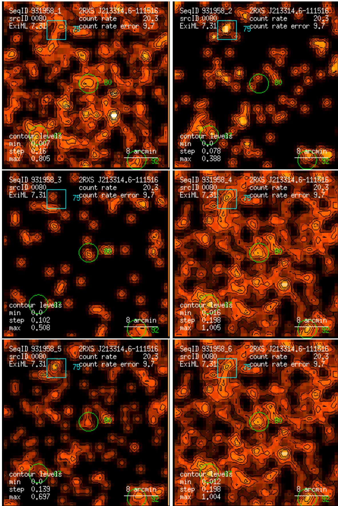
Figure 80: RASS 931958: detection 0080: band rate images, Gaussian filter: (1) PSPC channels 11 – 41, (2) 52 – 90, (3) 91 – 201, (4) 11 – 235, (5) 52 – 201, (6) 11 – 201. Broad band rates in counts/ks. Band rate contour levels in counts/ks/arcmin 2 .
