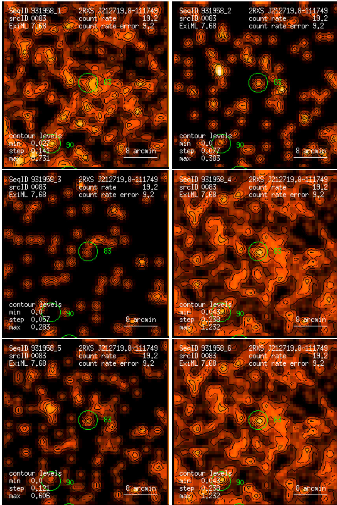
Figure 83: RASS 931958: detection 0083: band rate images, Gaussian filter: (1) PSPC channels 11 – 41, (2) 52 – 90, (3) 91 – 201, (4) 11 – 235, (5) 52 – 201, (6) 11 – 201. Broad band rates in counts/ks. Band rate contour levels in counts/ks/arcmin 2 .
