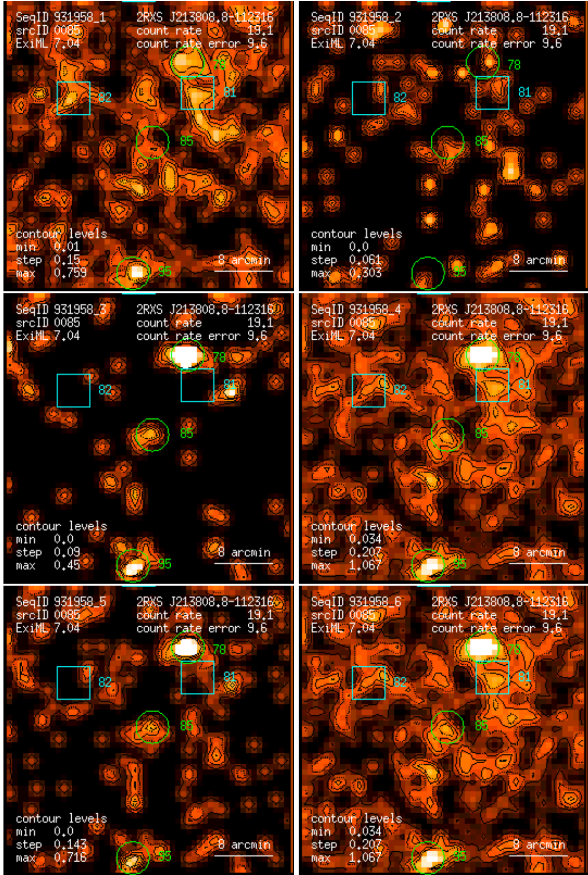
Figure 85: RASS 931958: detection 0085: band rate images, Gaussian filter: (1) PSPC channels 11 – 41, (2) 52 – 90, (3) 91 – 201, (4) 11 – 235, (5) 52 – 201, (6) 11 – 201. Broad band rates in counts/ks. Band rate contour levels in counts/ks/arcmin 2 .
