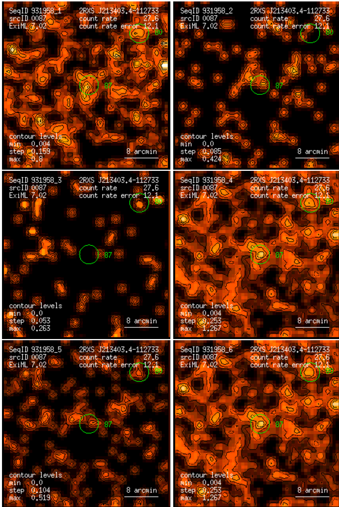
Figure 87: RASS 931958: detection 0087: band rate images, Gaussian filter: (1) PSPC channels 11 – 41, (2) 52 – 90, (3) 91 – 201, (4) 11 – 235, (5) 52 – 201, (6) 11 – 201. Broad band rates in counts/ks. Band rate contour levels in counts/ks/arcmin 2 .
