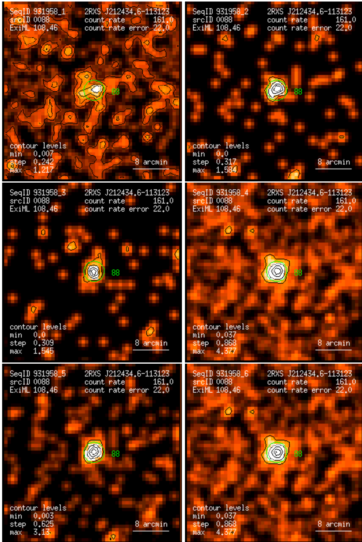
Figure 88: RASS 931958: detection 0088: band rate images, Gaussian filter: (1) PSPC channels 11 – 41, (2) 52 – 90, (3) 91 – 201, (4) 11 – 235, (5) 52 – 201, (6) 11 – 201. Broad band rates in counts/ks. Band rate contour levels in counts/ks/arcmin 2 .
