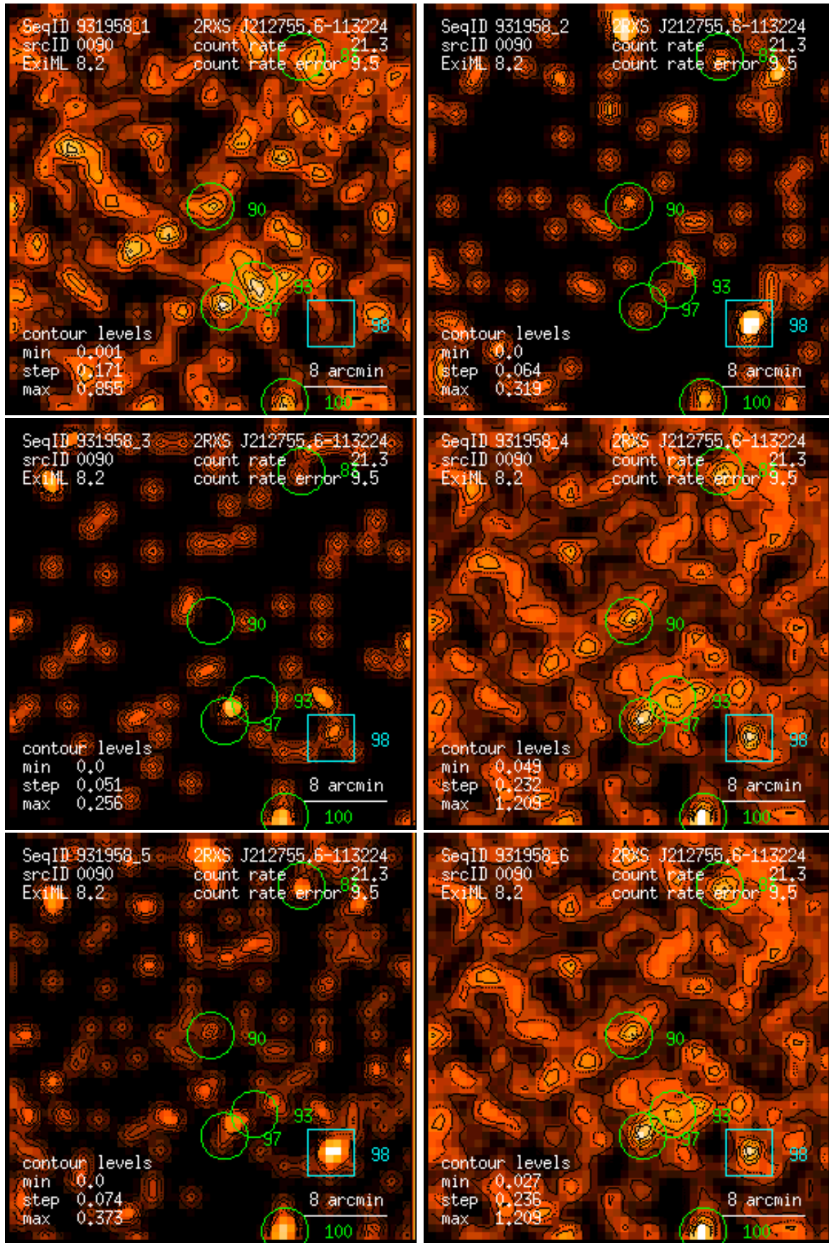
Figure 90: RASS 931958: detection 0090: band rate images, Gaussian filter: (1) PSPC channels 11 – 41, (2) 52 – 90, (3) 91 – 201, (4) 11 – 235, (5) 52 – 201, (6) 11 – 201. Broad band rates in counts/ks. Band rate contour levels in counts/ks/arcmin 2 .
