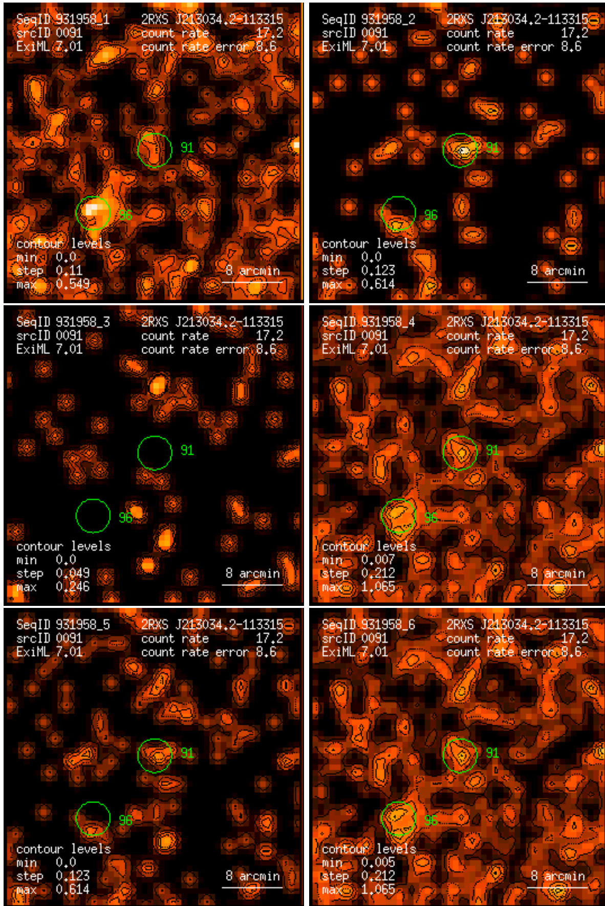
Figure 91: RASS 931958: detection 0091: band rate images, Gaussian filter: (1) PSPC channels 11 – 41, (2) 52 – 90, (3) 91 – 201, (4) 11 – 235, (5) 52 – 201, (6) 11 – 201. Broad band rates in counts/ks. Band rate contour levels in counts/ks/arcmin 2 .
