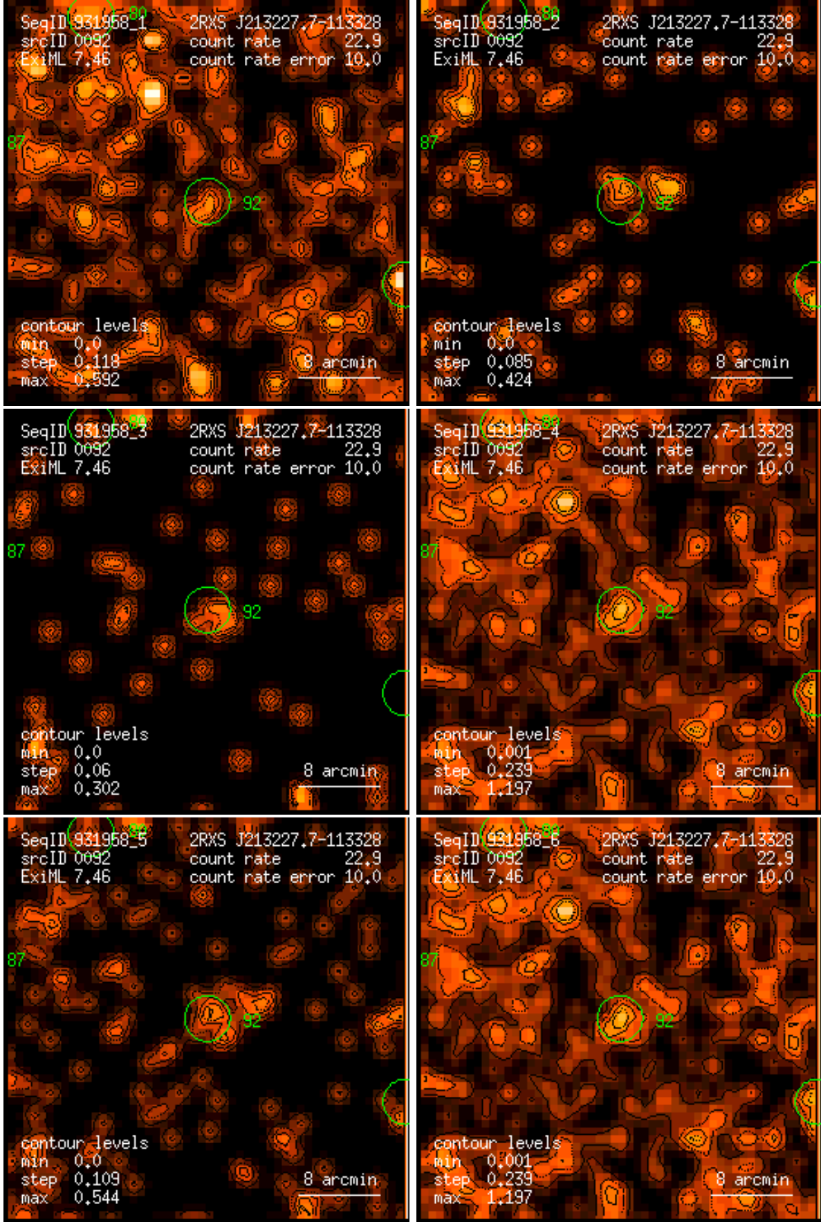
Figure 92: RASS 931958: detection 0092: band rate images, Gaussian filter: (1) PSPC channels 11 – 41, (2) 52 – 90, (3) 91 – 201, (4) 11 – 235, (5) 52 – 201, (6) 11 – 201. Broad band rates in counts/ks. Band rate contour levels in counts/ks/arcmin 2 .
