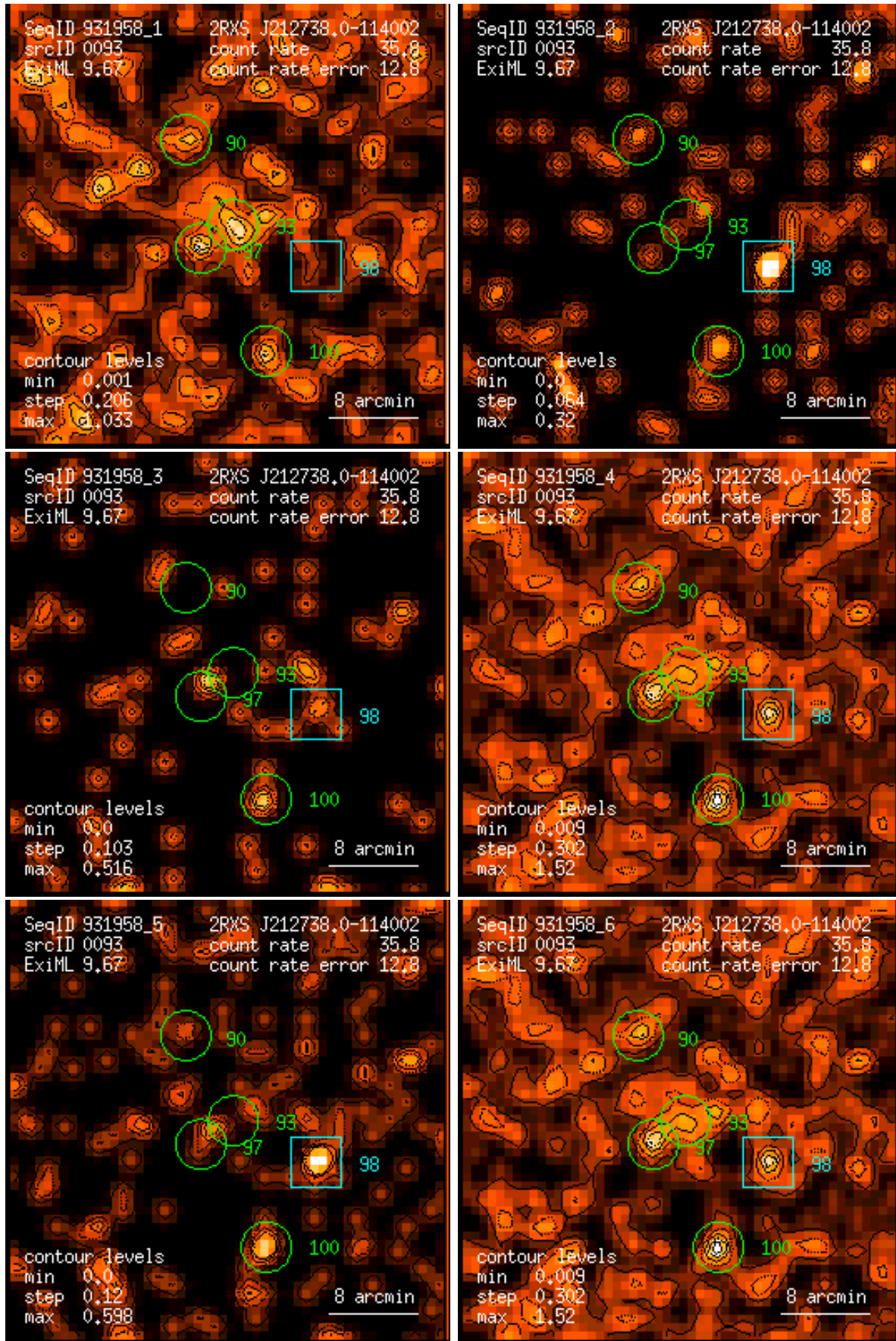
Figure 93: RASS 931958: detection 0093: band rate images, Gaussian filter: (1) PSPC channels 11 – 41, (2) 52 – 90, (3) 91 – 201, (4) 11 – 235, (5) 52 – 201, (6) 11 – 201. Broad band rates in counts/ks. Band rate contour levels in counts/ks/arcmin 2 .
