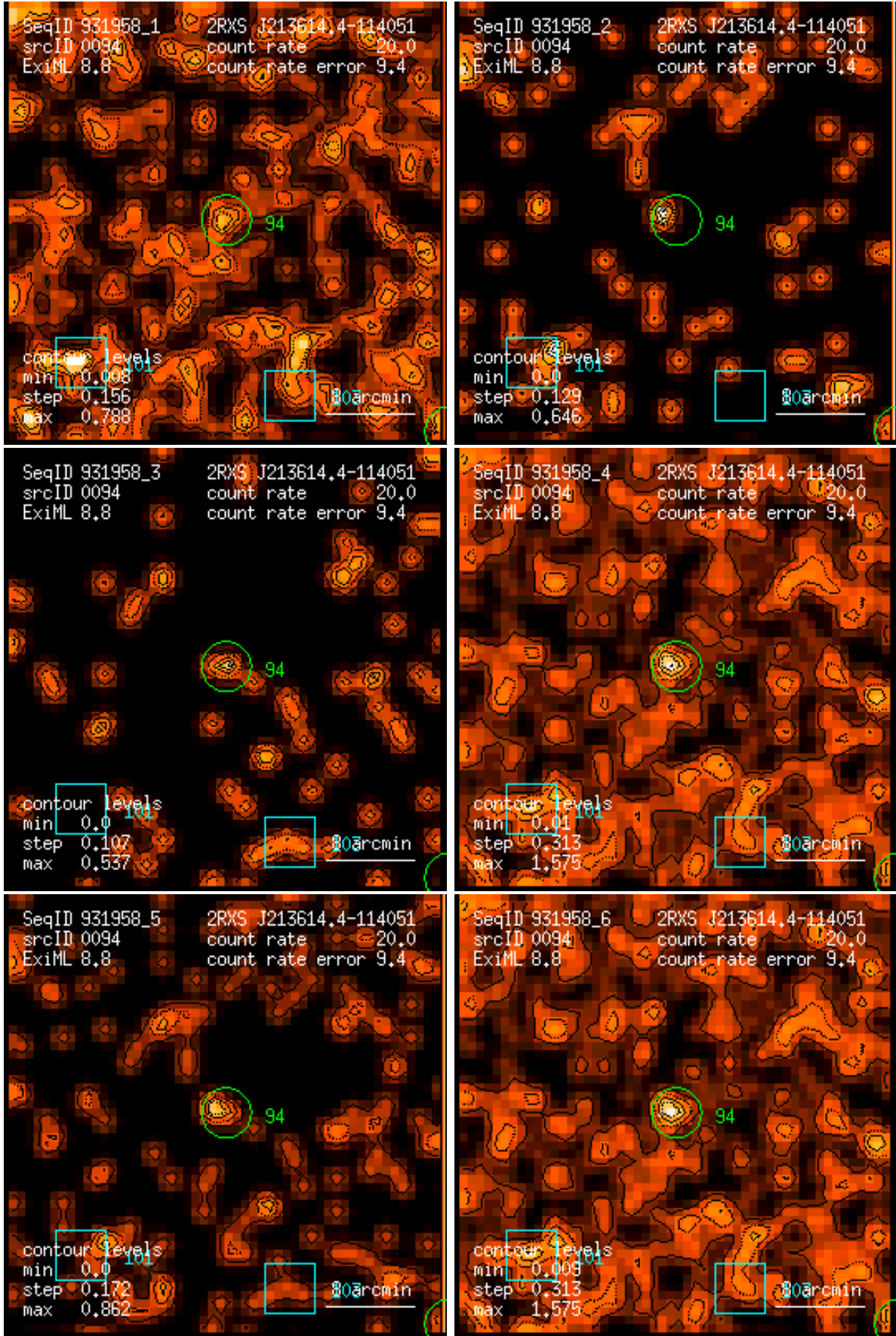
Figure 94: RASS 931958: detection 0094: band rate images, Gaussian filter: (1) PSPC channels 11 – 41, (2) 52 – 90, (3) 91 – 201, (4) 11 – 235, (5) 52 – 201, (6) 11 – 201. Broad band rates in counts/ks. Band rate contour levels in counts/ks/arcmin 2 .
